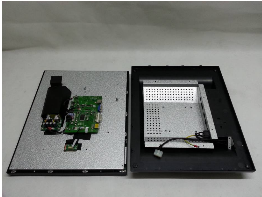
INTERNAL PHOTO OF SAMPLE-HL1916SM -1
