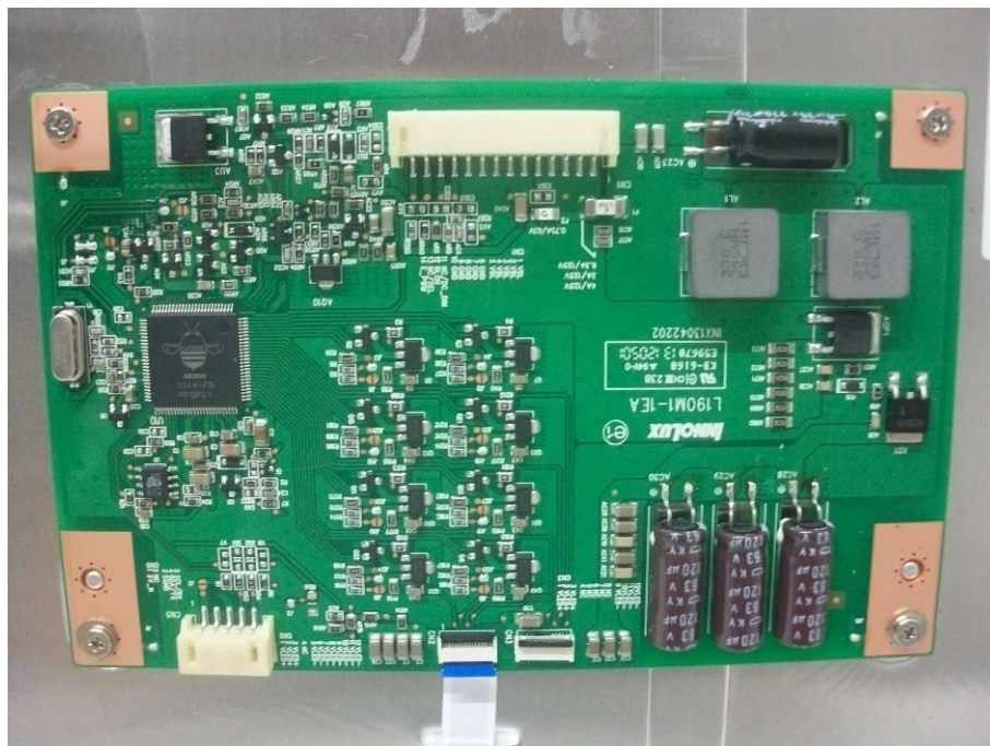
INTERNAL PHOTO OF SAMPLE-HL1916AMT-R -2
