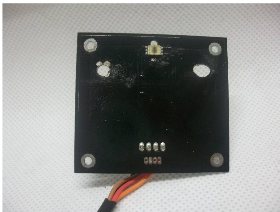
INTERNAL PHOTO OF SAMPLE-HL1916 -9
