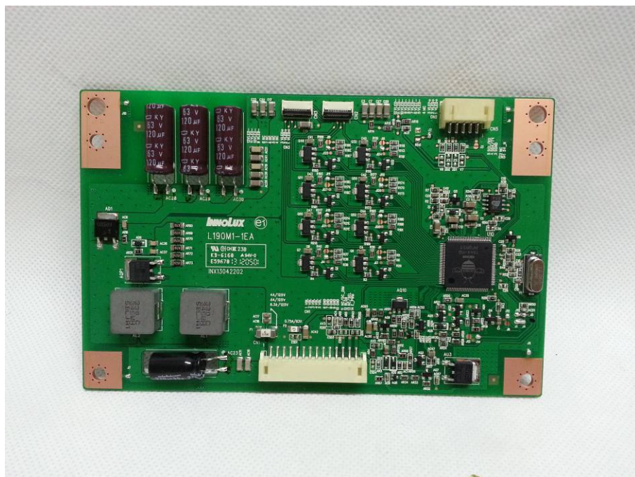
INTERNAL PHOTO OF SAMPLE-HL1916SM -2
