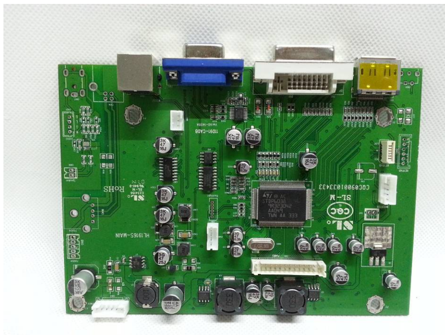
INTERNAL PHOTO OF SAMPLE-HL1916SM -4
