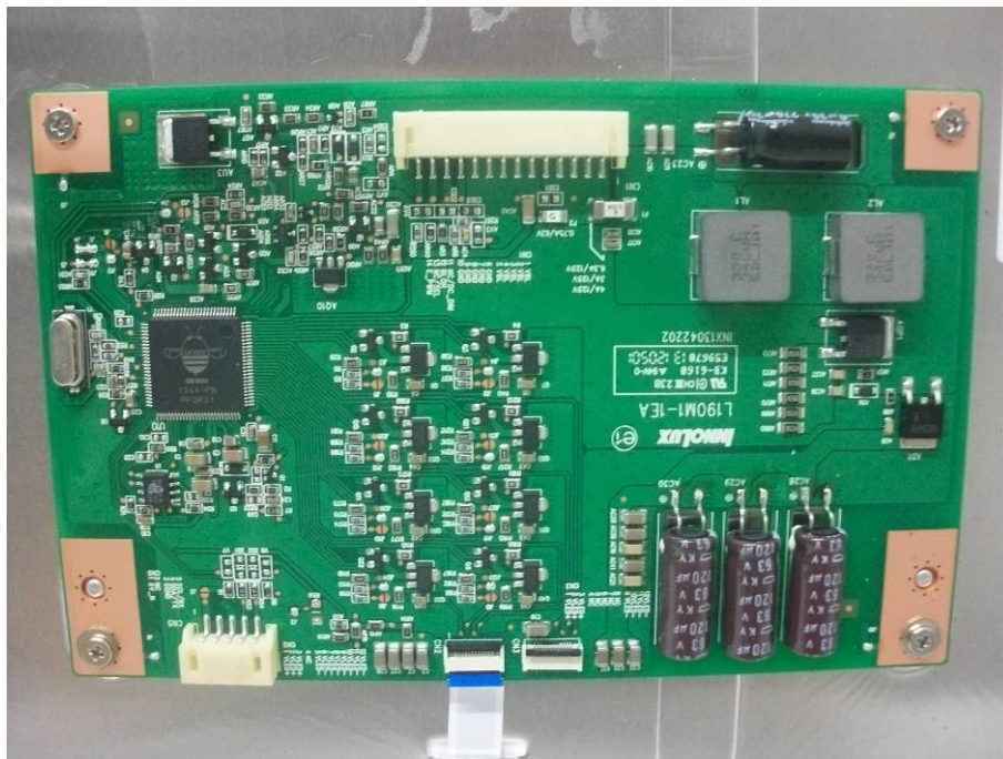
INTERNAL PHOTO OF SAMPLE-HL1916 -2
