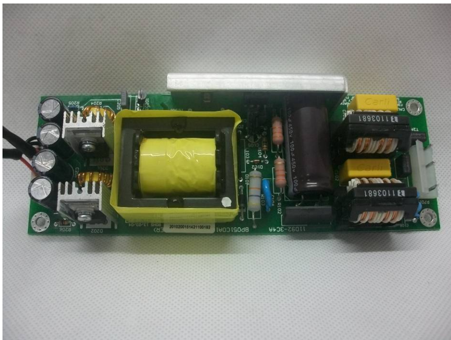
INTERNAL PHOTO OF SAMPLE-HL1916SM -10
