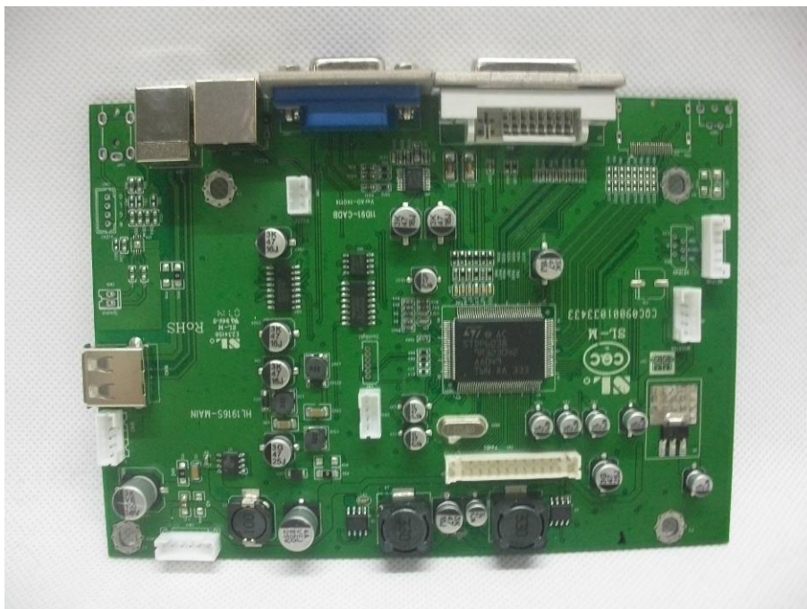
INTERNAL PHOTO OF SAMPLE-HL1916AMT-R -4
