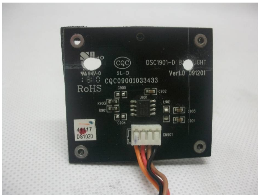
INTERNAL PHOTO OF SAMPLE-HL1916AMT-R -8
