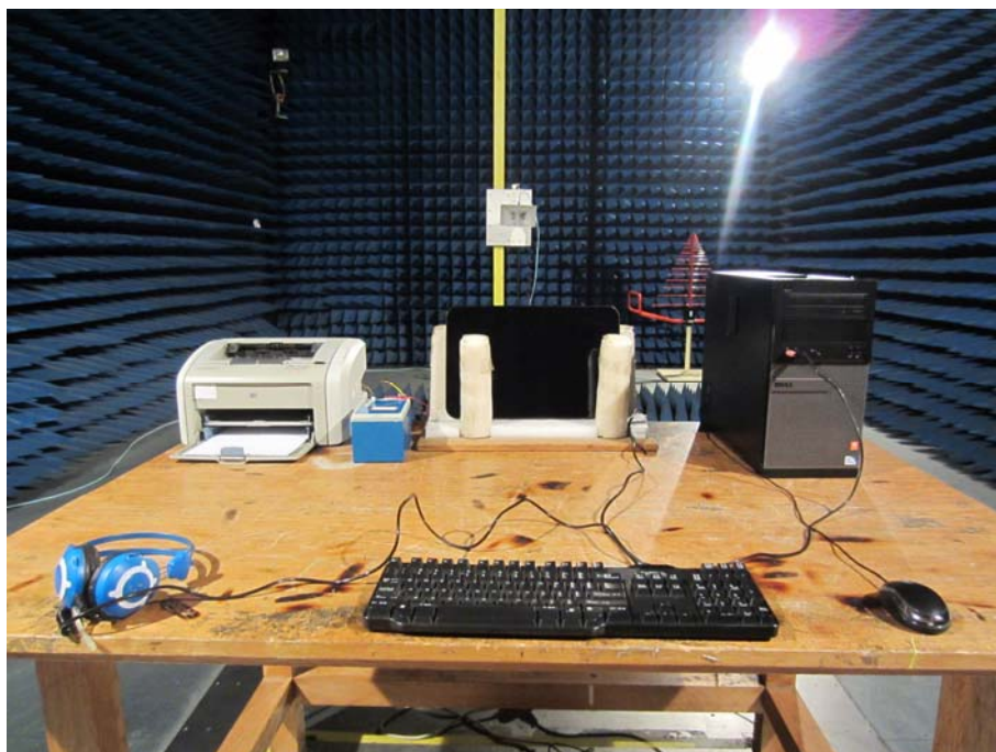
RE TEST SETUP OF HL1530
