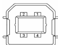
Figure 2.4 USB-B connector
