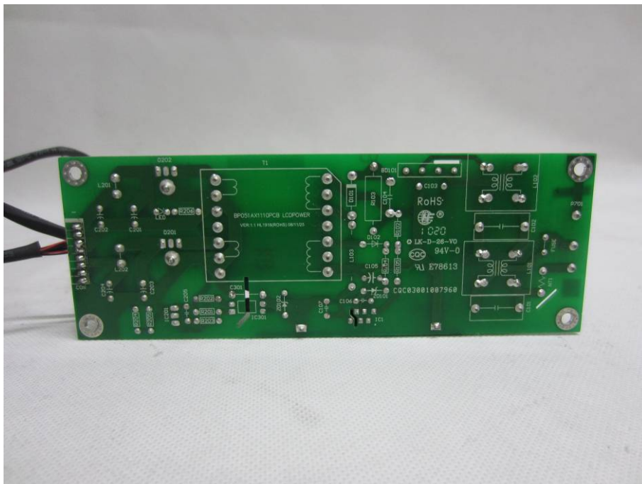
INTERNAL PHOTO OF SAMPLE-C15S -6
