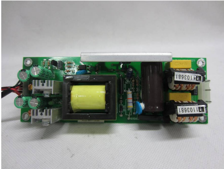
INTERNAL PHOTO OF SAMPLE-C15S -5
