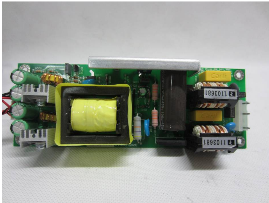
INTERNAL PHOTO OF SAMPLE-HL1916BT -7
