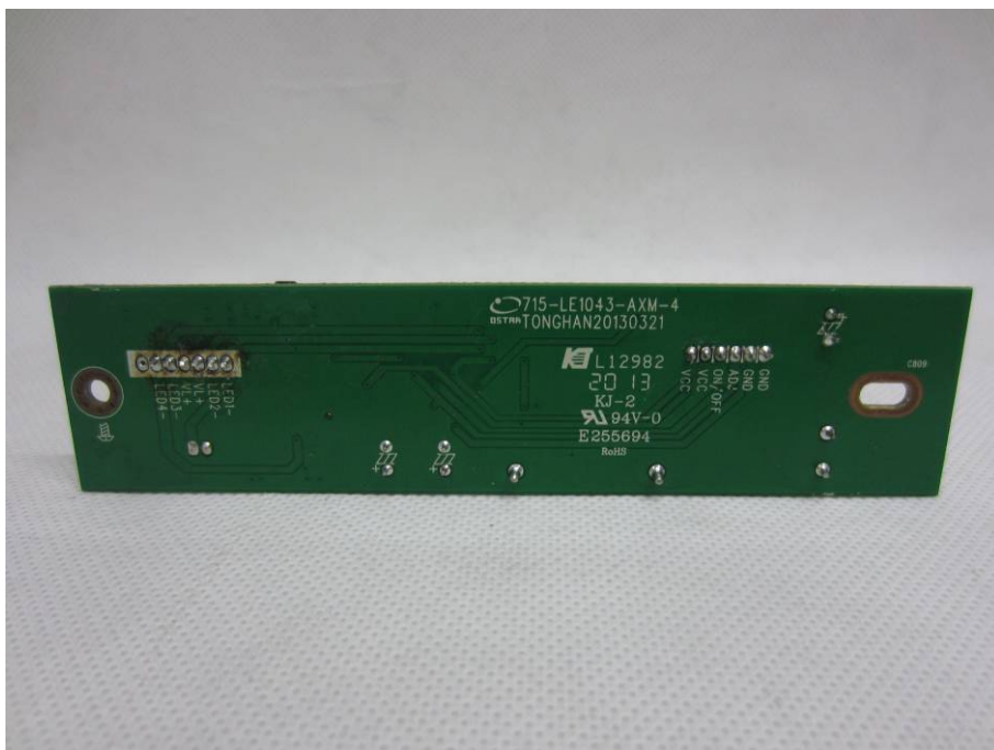
INTERNAL PHOTO OF SAMPLE-HL1916LA -8
