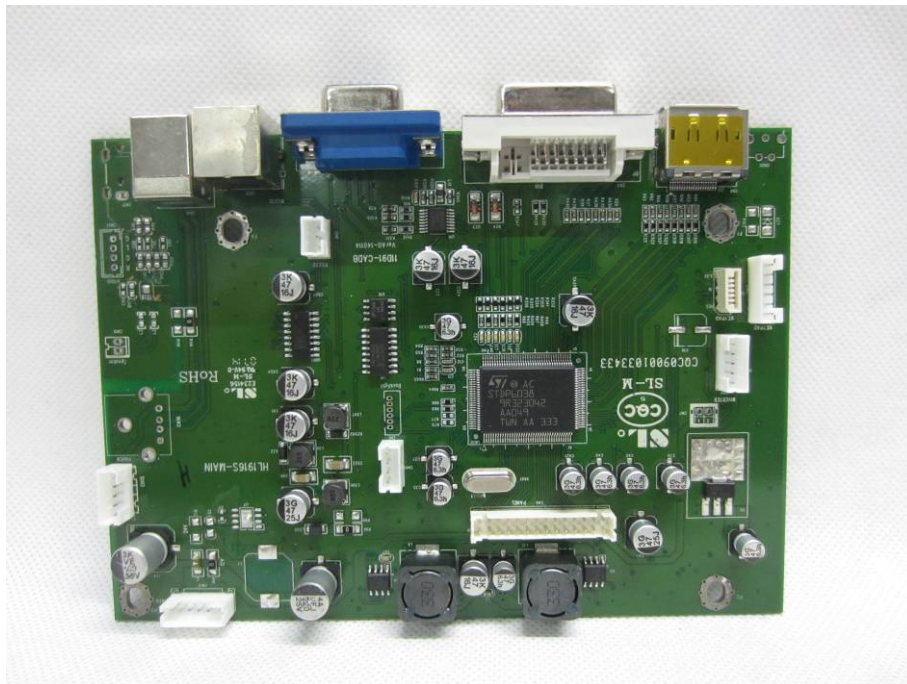
INTERNAL PHOTO OF SAMPLE-HL1916BT -3
