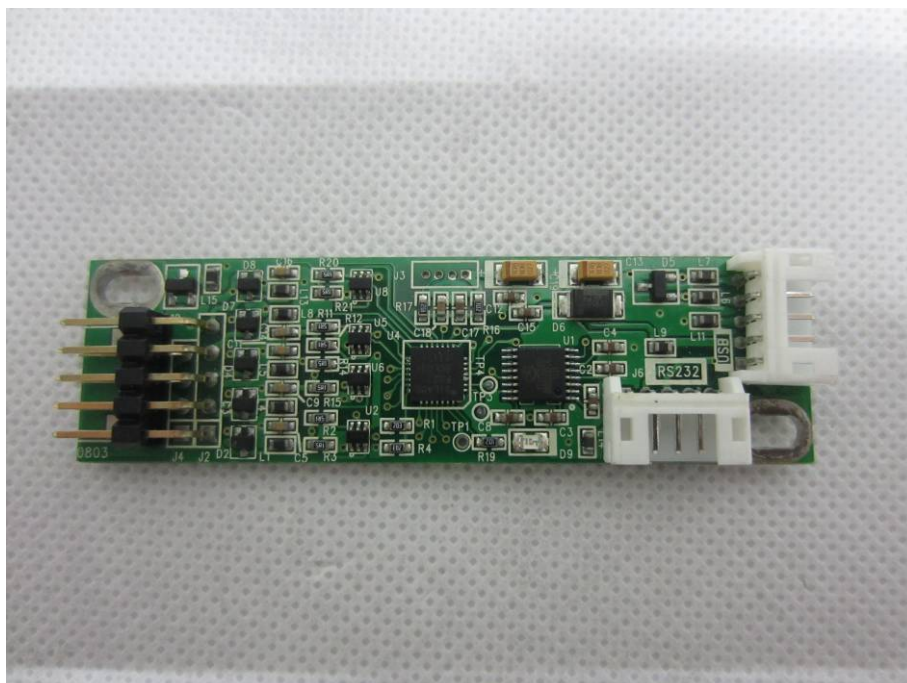
INTERNAL PHOTO OF SAMPLE-HL1916BT -6
