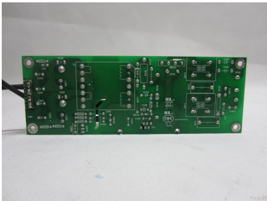
INTERNAL PHOTO OF SAMPLE-HL1916BT -8
