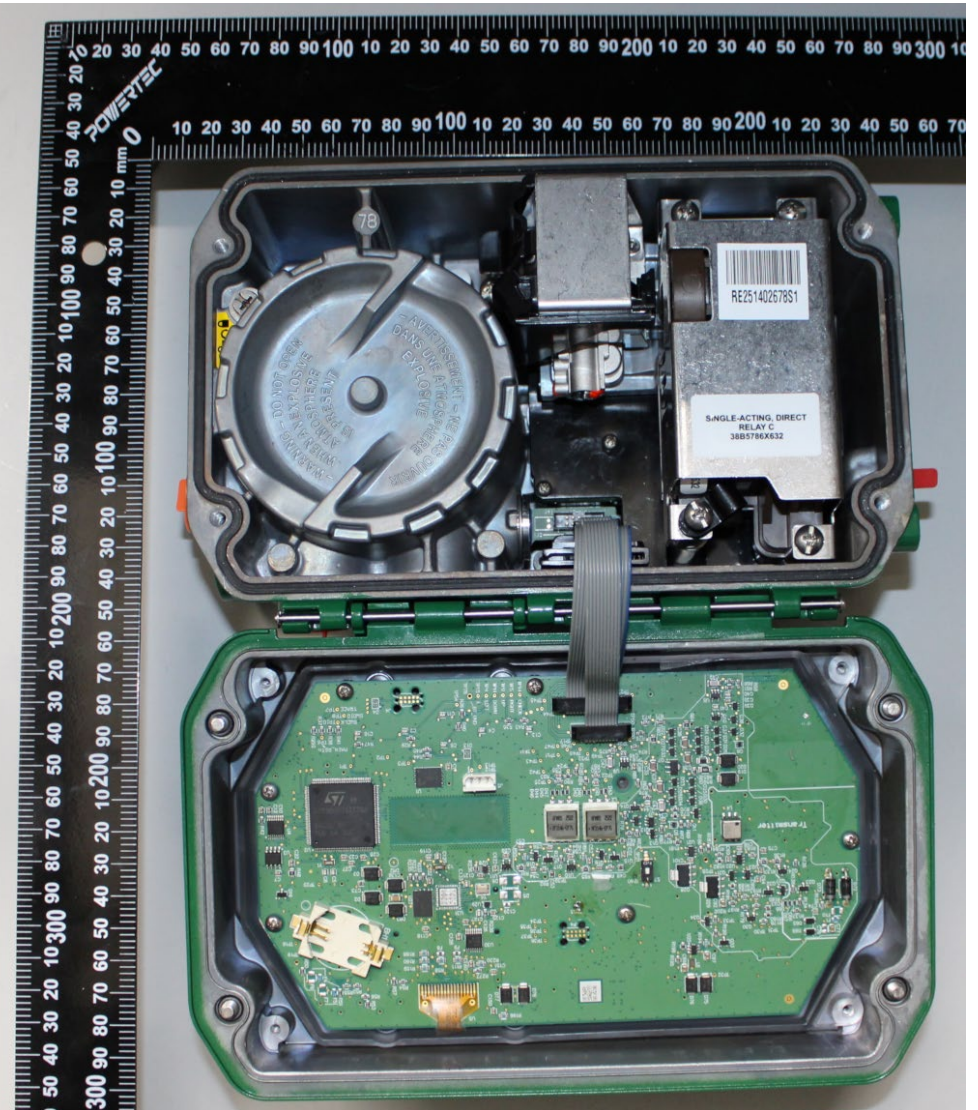
Front View (full cover open) – See page 4 for board photo
