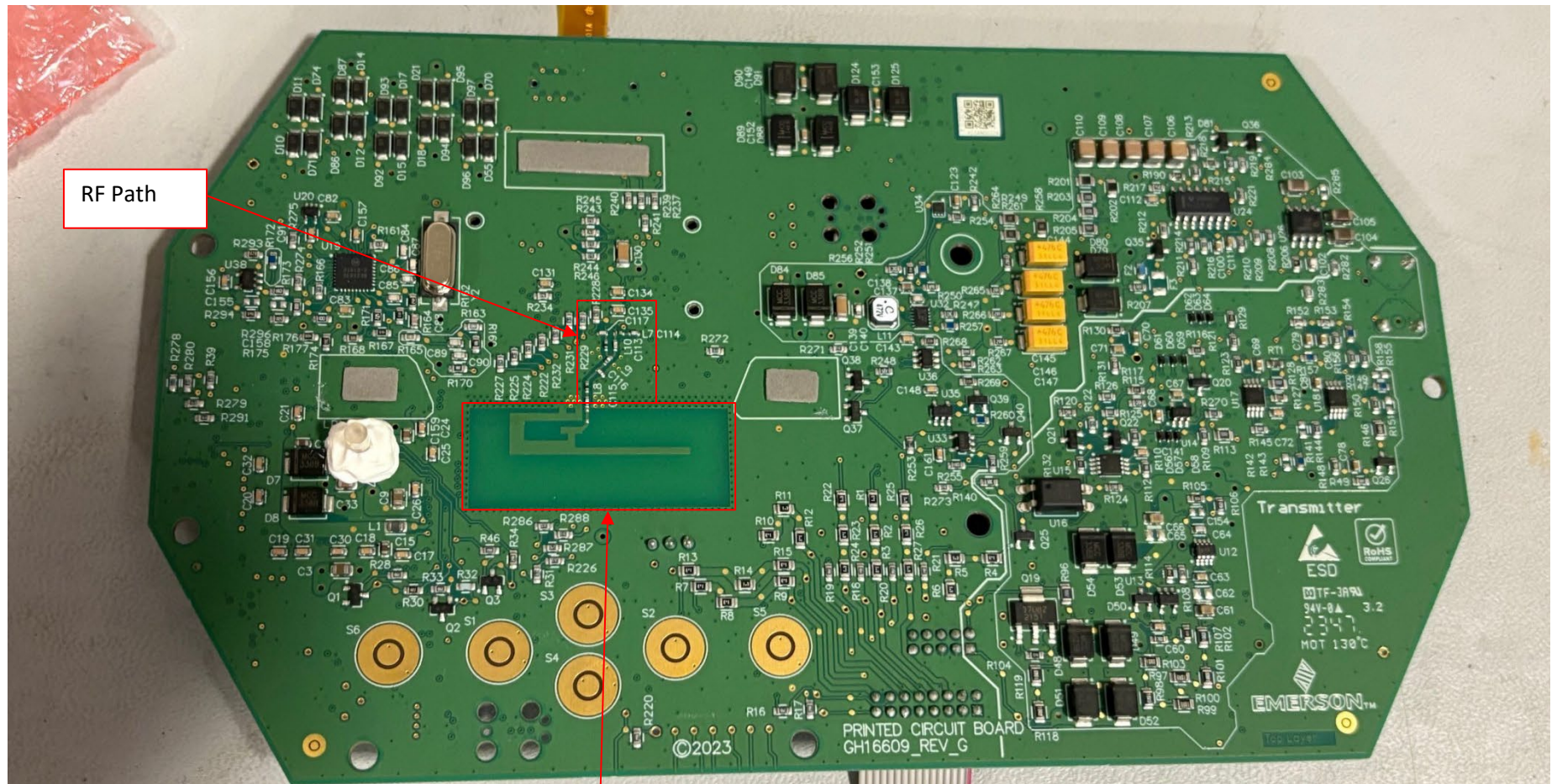
PCB Trace Antenna
