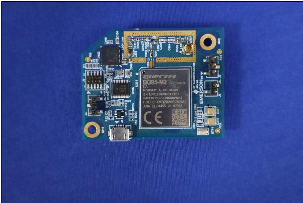
RF Module PCB Front View
