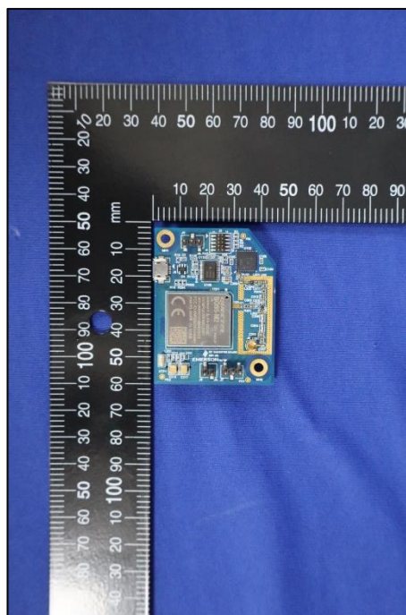
PCB Dimensional View
