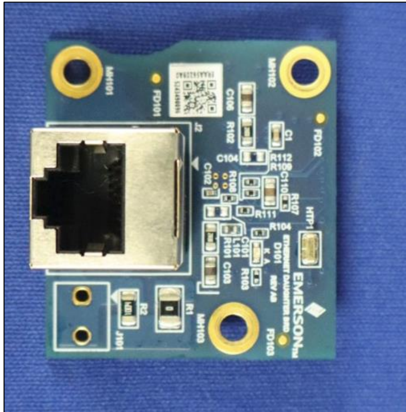
Ethernet Daughter Board PCB front View
