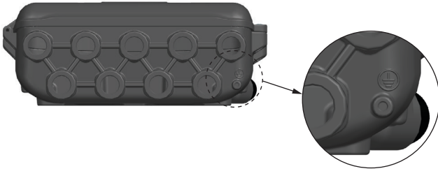
Figure 2. ARMOR Enclosure Grounding Location
