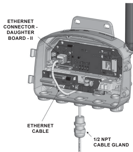
Figure 15. Ethernet Installation
