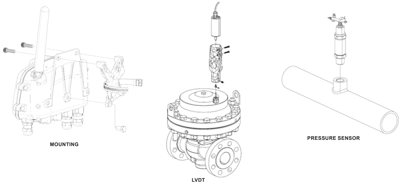
Figure 3. Installation Procedures
