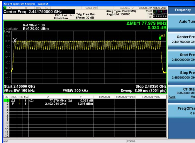
GFSK Modulation
