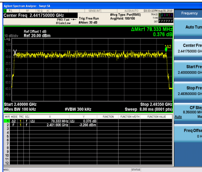
8DPSK Modulation
