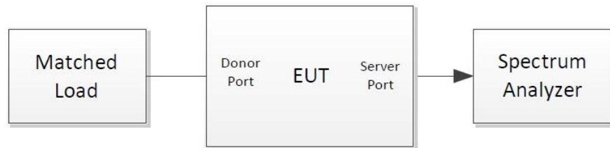
Figure 6 – Maximum downlink noise limit test configuration
