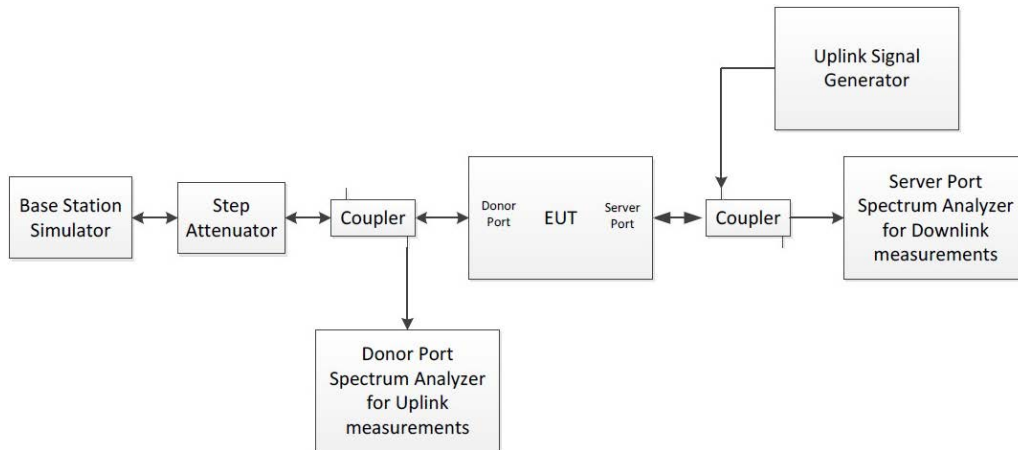
Figure 1 – Test configuration in EUT normal operational mode
