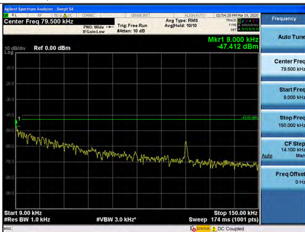
Spurious / BRS/EBS / Downlink / 5G NR 60M / Low / 9 kHz ~ 150 kHz
