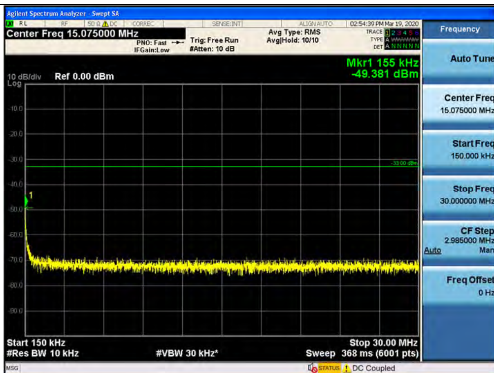
Spurious / BRS/EBS / Downlink / 5G NR 60M / Low / 150 kHz ~ 30 MHz
