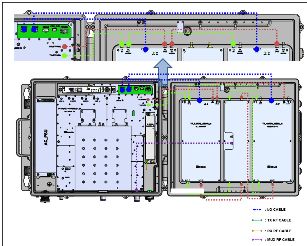
Figure 4.16 – Cabling of N2RDU_1900P_M + N2RDU_L2600F_M or N2RDU_AWS13_M + N2RDU_L2600F_M (MIMO Band Expansion)
