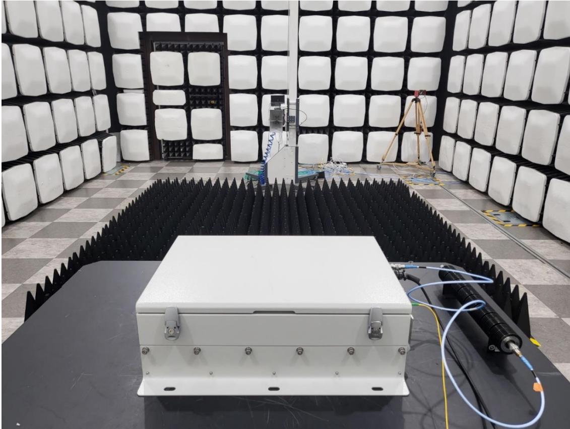
[HRDU_2500_Veritical(Enclosure)]
