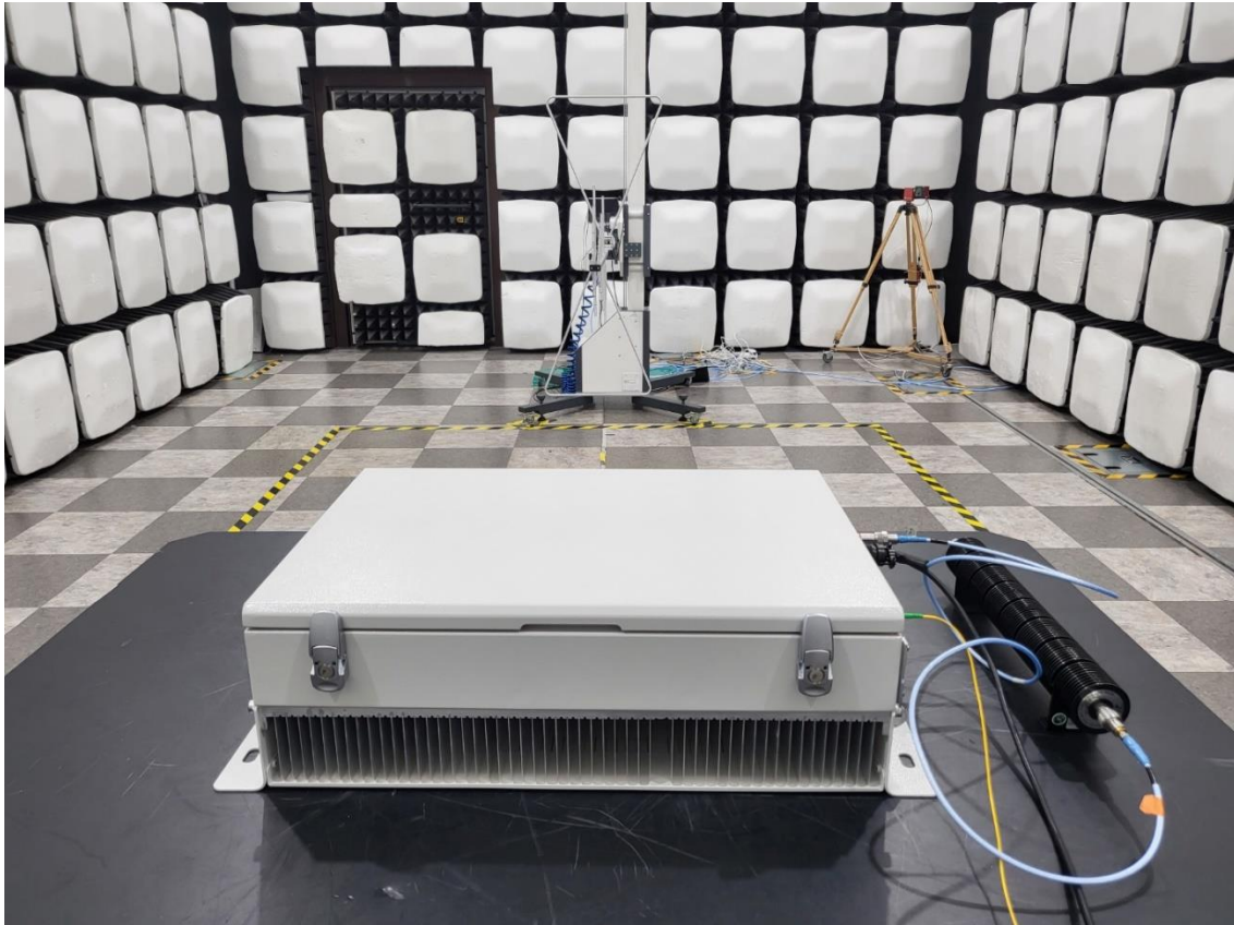
[HRDU_2500_Horizontal(Enclosure)]
