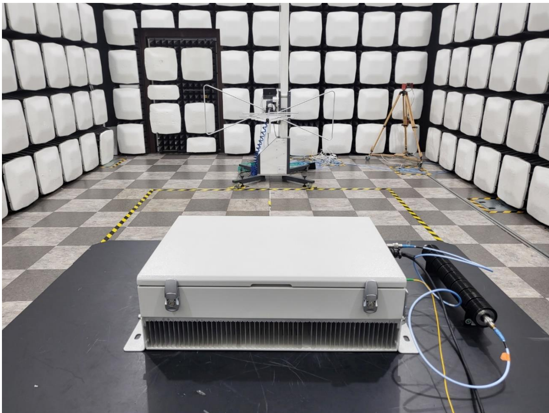
[HRDU_2500_Horizontal(Enclosure)]
