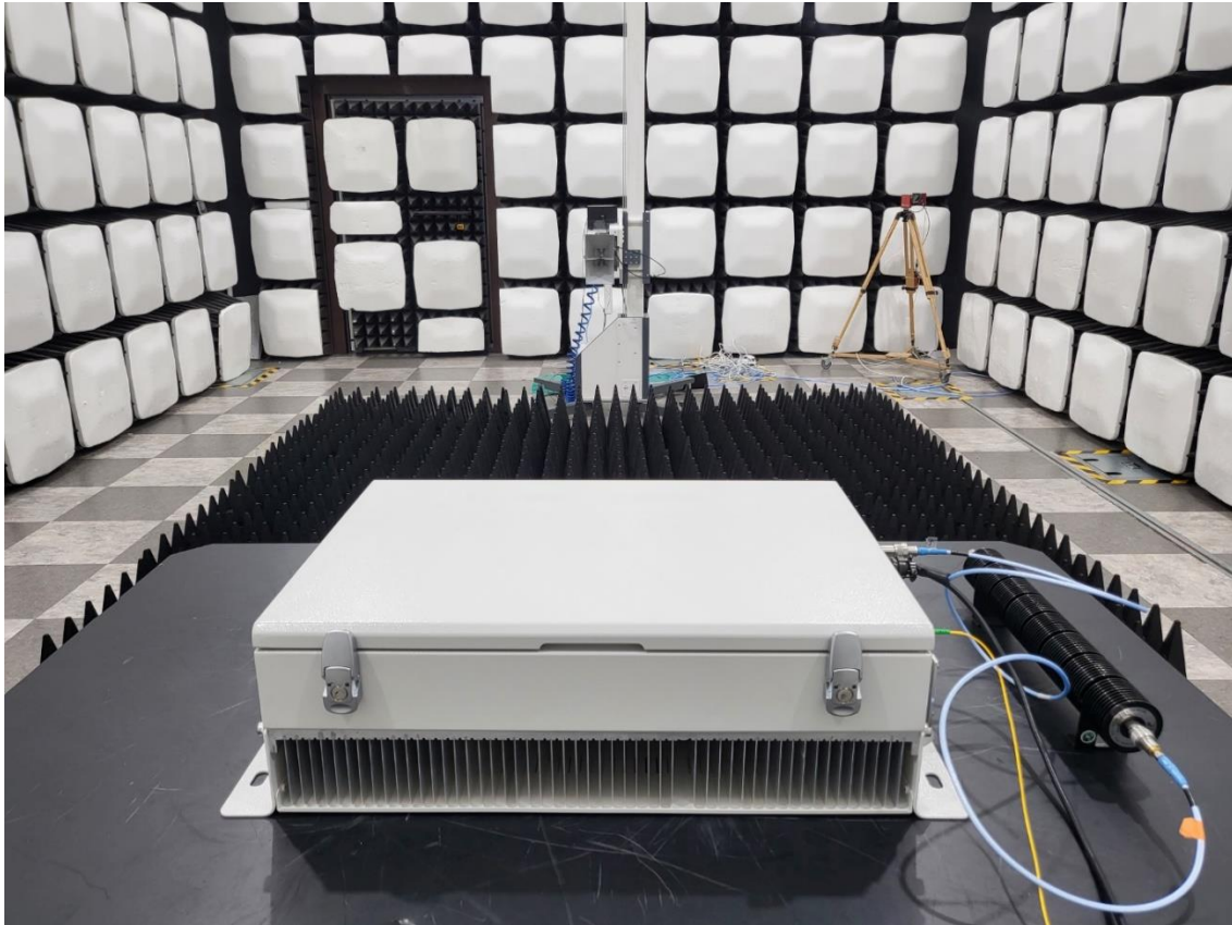
[HRDU_2500_Horizontal(Enclosure)]
