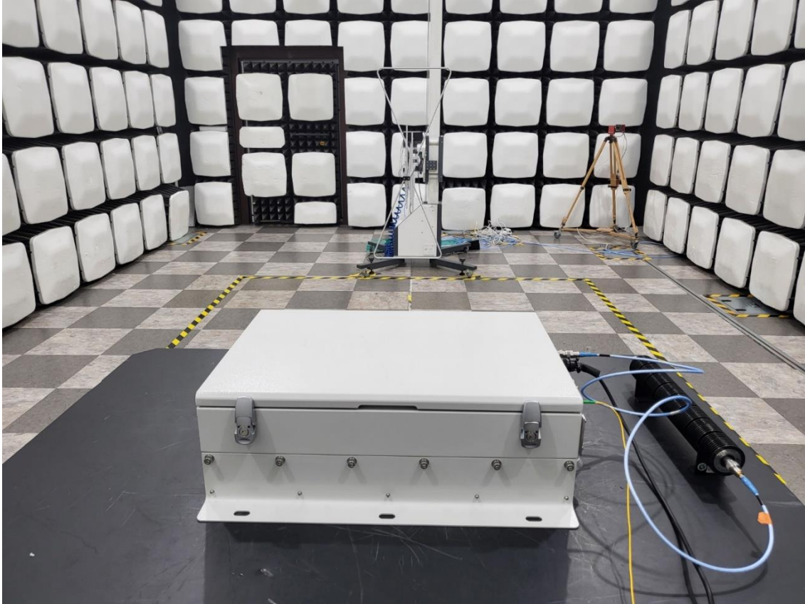
[HRDU_2500_Vertical(Enclosure)]
