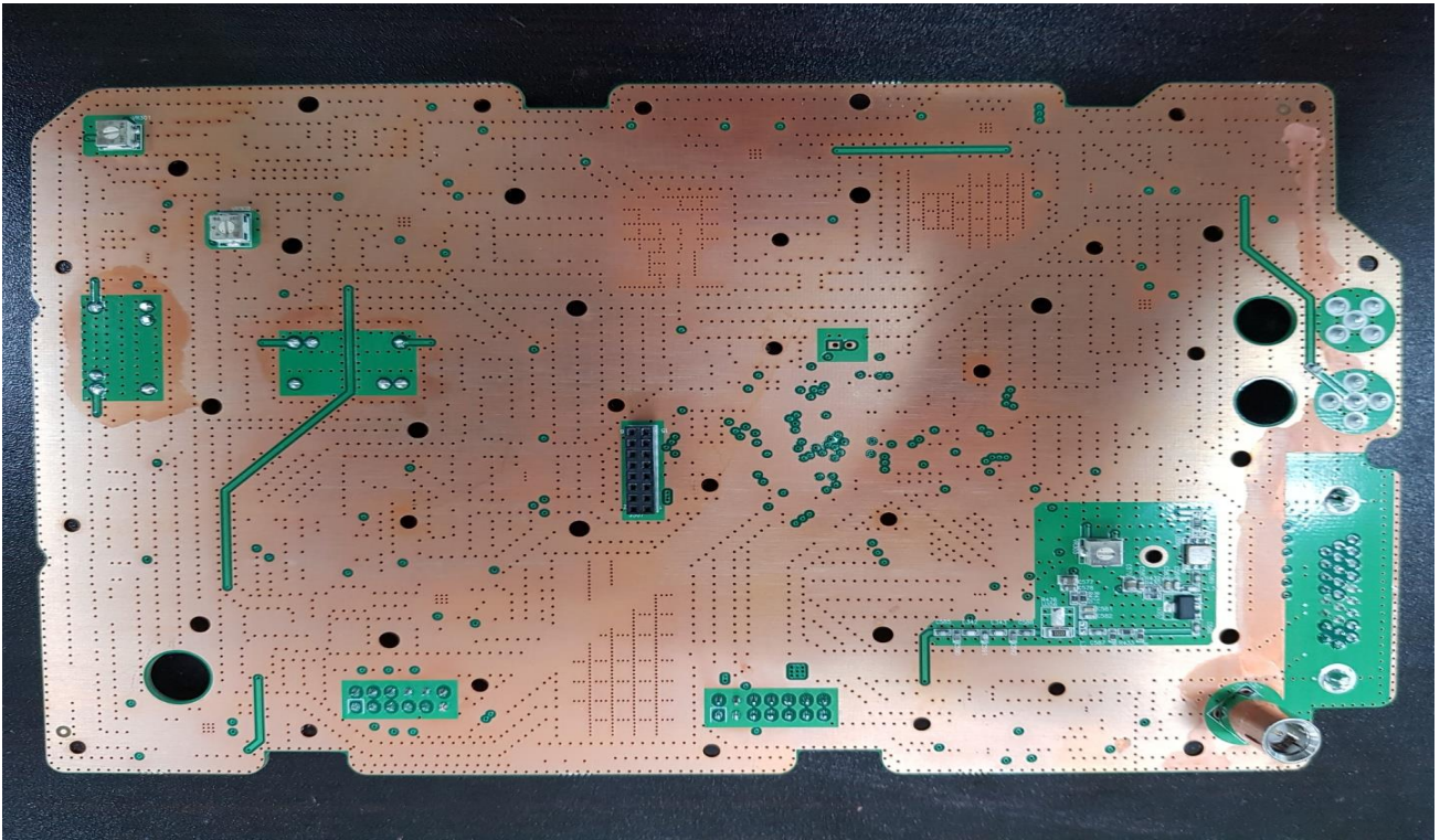
[UDCU RX PBA Bottom]
