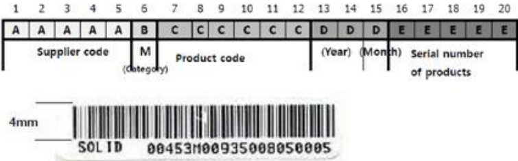
(nMRFM_17,19,23,25,34)
