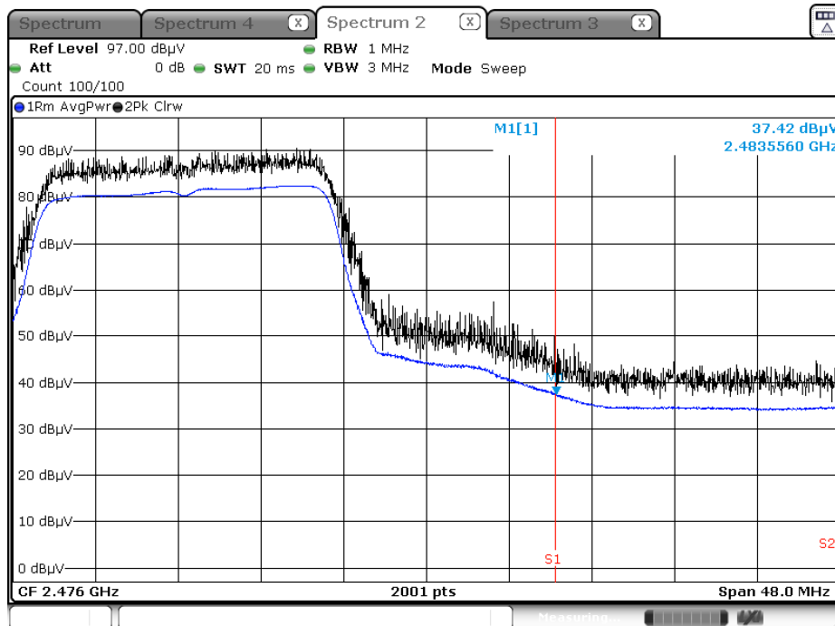
Radiated Restricted Band Edges plot – Average Result (802.11g_6 Mbps, Ch.11, Y-H)
