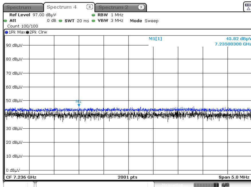
Radiated Spurious Emissions plot – Peak Result (802.11b_1 Mbps, Ch.1 3rd Harmonic, X-V)
