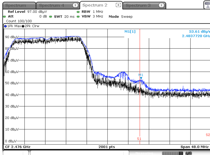
Radiated Restricted Band Edges plot – Peak Result (802.11g_6 Mbps, Ch.11, Y-H)
