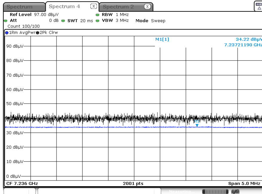
Radiated Spurious Emissions plot – Average Result (802.11b_1 Mbps, Ch.1 3rd Harmonic, X-V)
