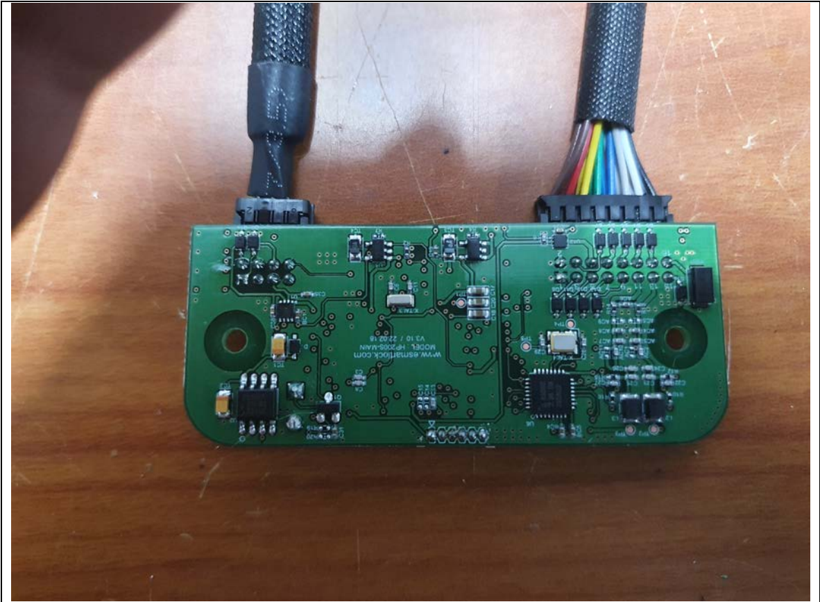
MainBoard-Rear
