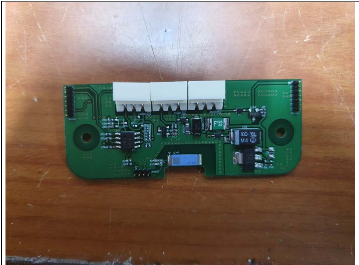
MainBoard-Rear
