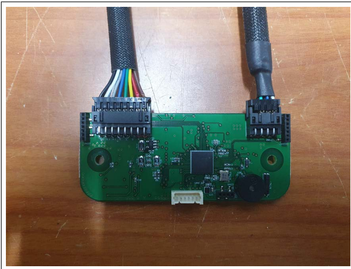
MainBoard-Rear
