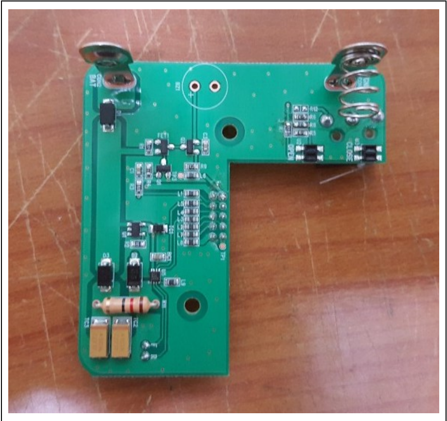
SubBoard-Rear
