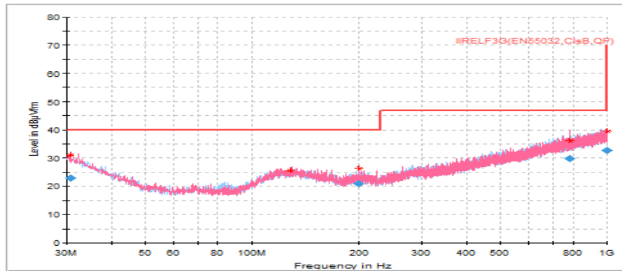
Figure B1: Radiated Emissions 30M-1G Hz for FCC/ISED - 120V/60H - RX
