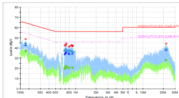
Figure A2: AC Mains Conducted Emissions for FCC/ISED - 120V/60H - TX Worst-Case - L1/L2
