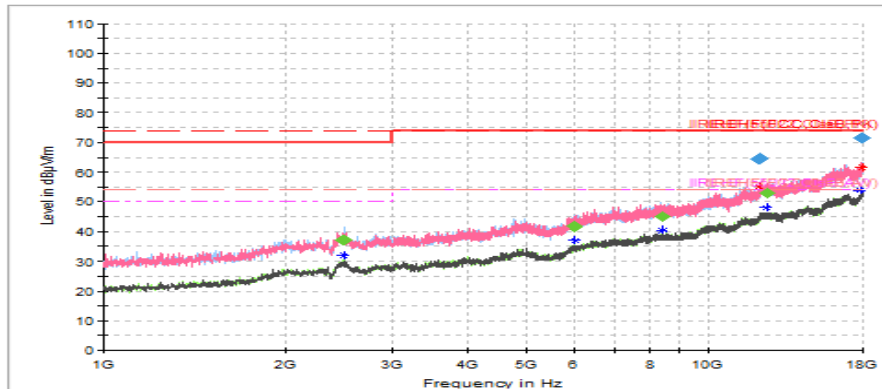
Figure B4: Radiated Emissions 1G-18G Hz for FCC/ISED - 120V/60H - TX Worst-Case
