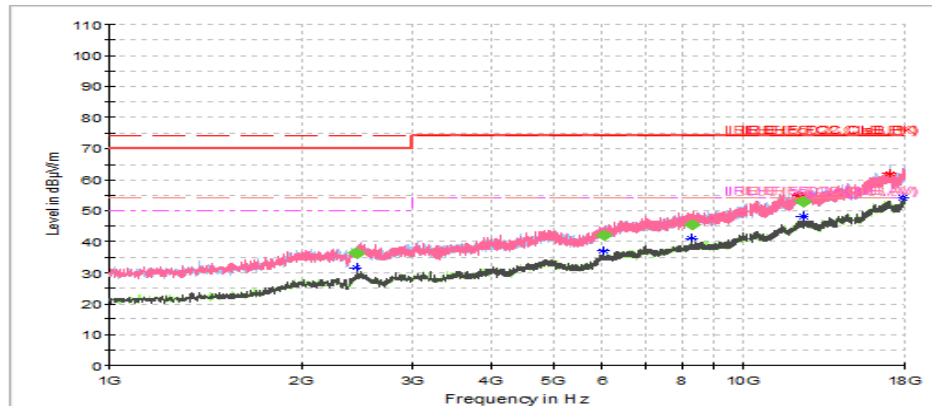
Figure B2: Radiated Emissions 1G-18G Hz for FCC/ISED - 120V/60H - RX
