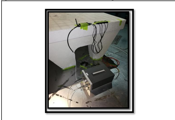
Figure R3: Conducted Emissions Test Setup
