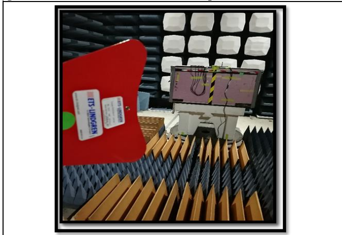
Figure R4: Radiated Emissions Test Setup
