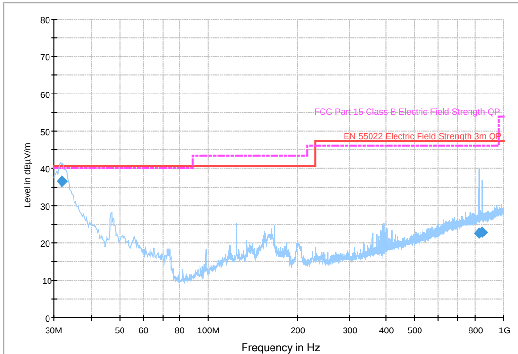
Radiated Spurious Emissions Plot: 30MHz – 1GHz_Modulation 802.11b, Channel 6
