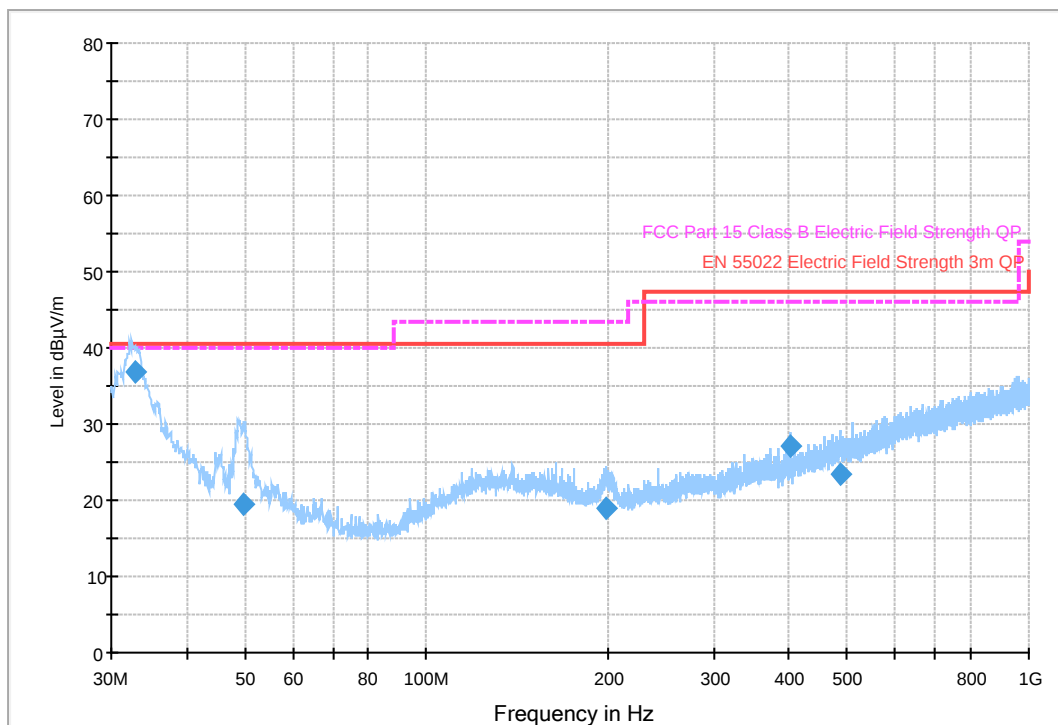
Radiated Spurious Emissions Plot: 30MHz – 1GHz_Modulation 802.11b, Channel 11
