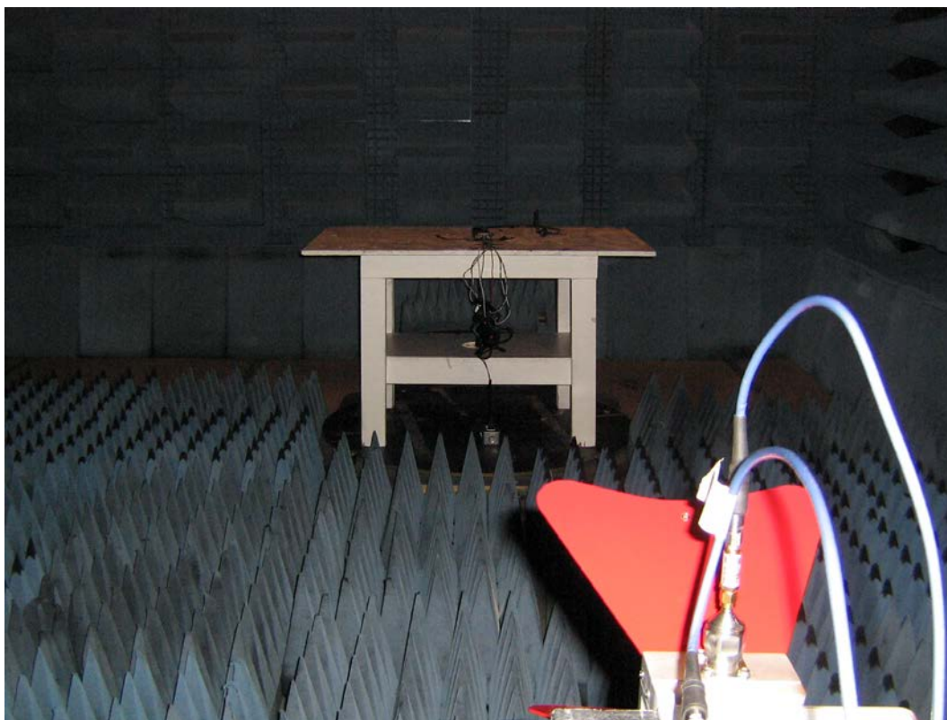
Radiated Emission Test Setup – 1GHz- 18GHz
