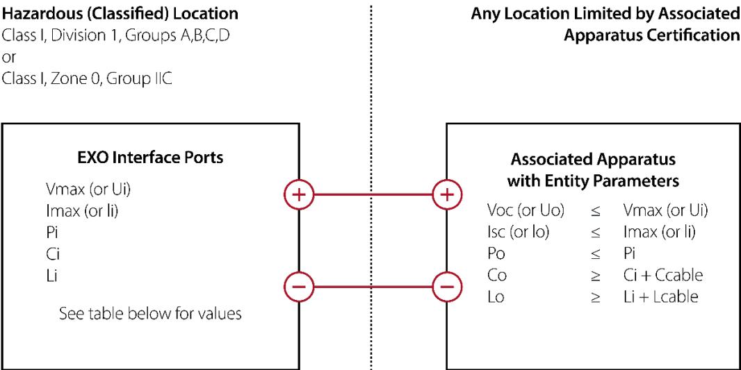
Input entity parameters (low side switch)
