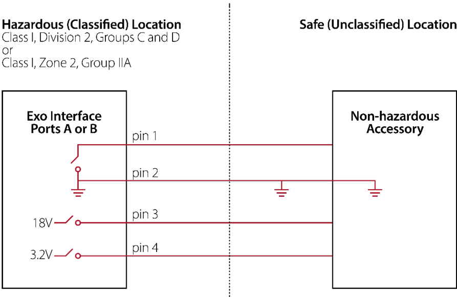
Diagram 13.5.5 Interface port functional parameters
