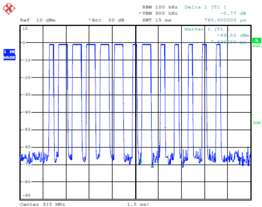
The graph shows the duration of ‘on’ signal. From marker 1 to marker 2, duration is 0.78ms.
