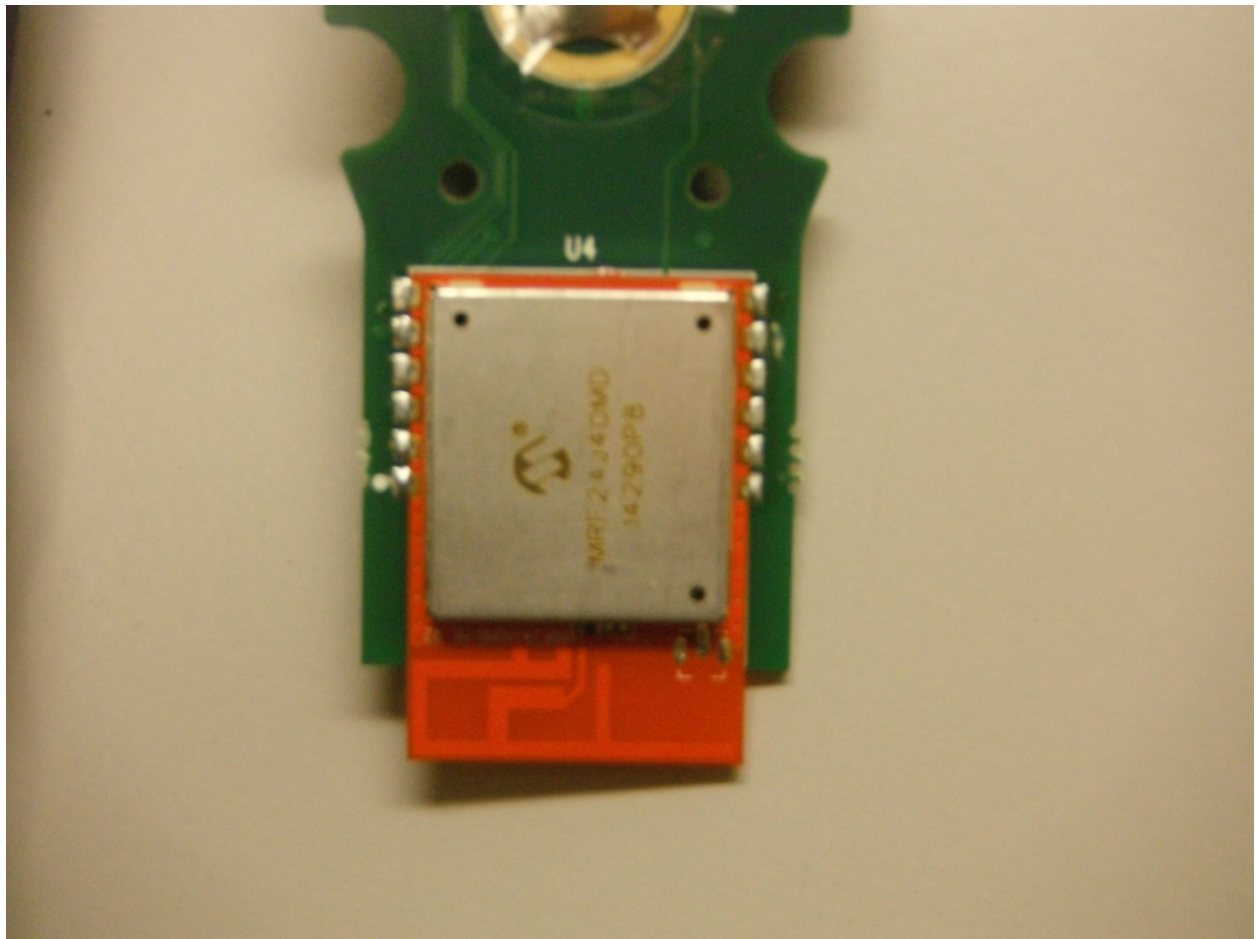
Figure 10: RF Module view
