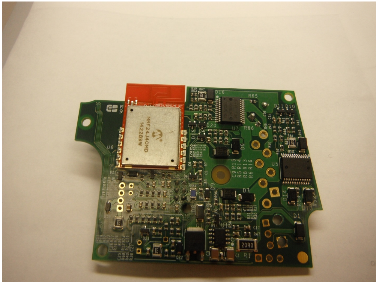
Figure 5: PCBA – Bottom view – RF Module
