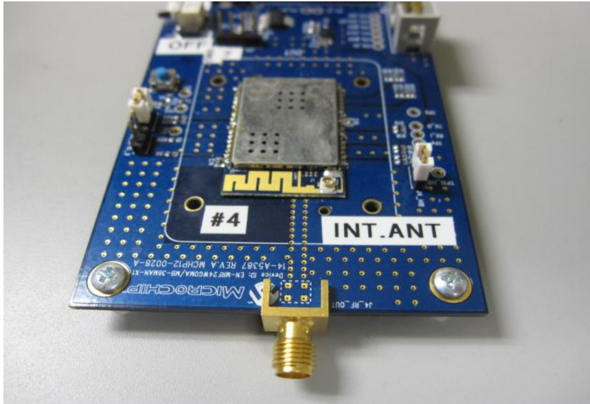
INTEGRAL ANTENNA
