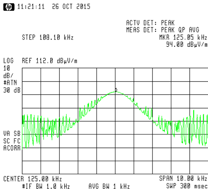
Figure 8. Field Strength of Fundamental, Low Detector: Peak
