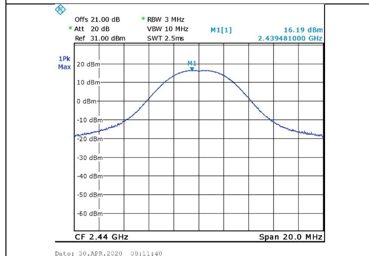
Figure 24. 2440.0 MHz
