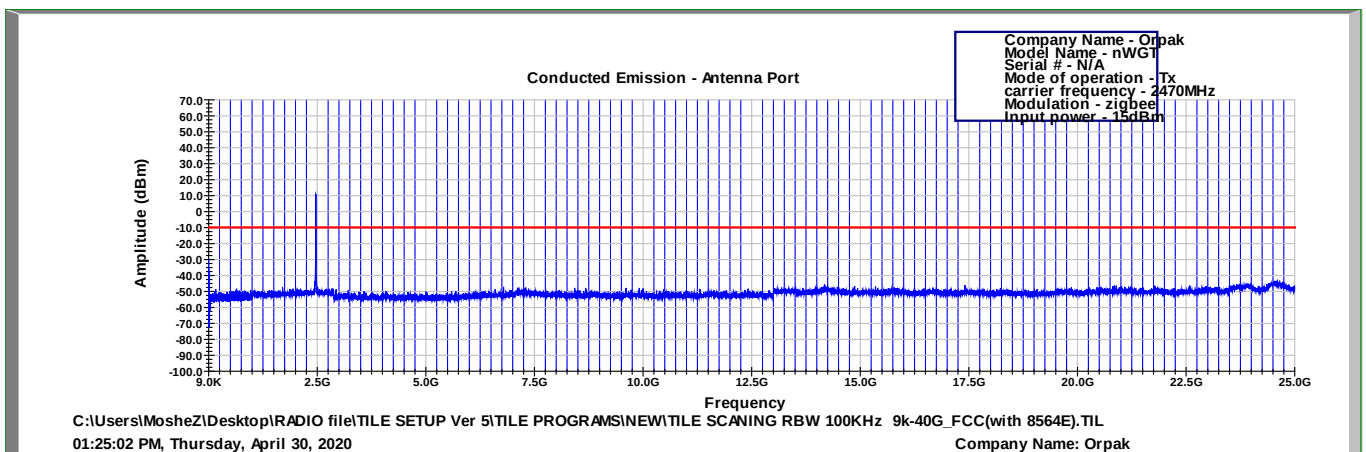
Figure 43 2470.0 MHz
