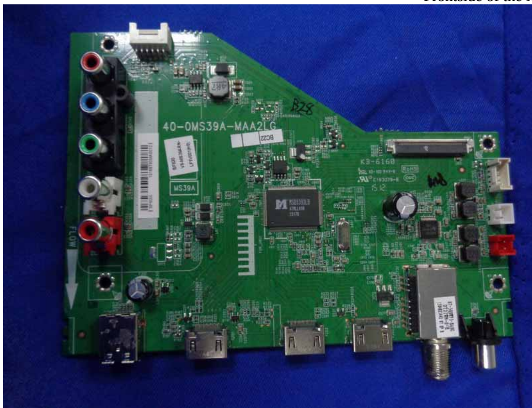
Figure 7 Frontside of the Main Board
