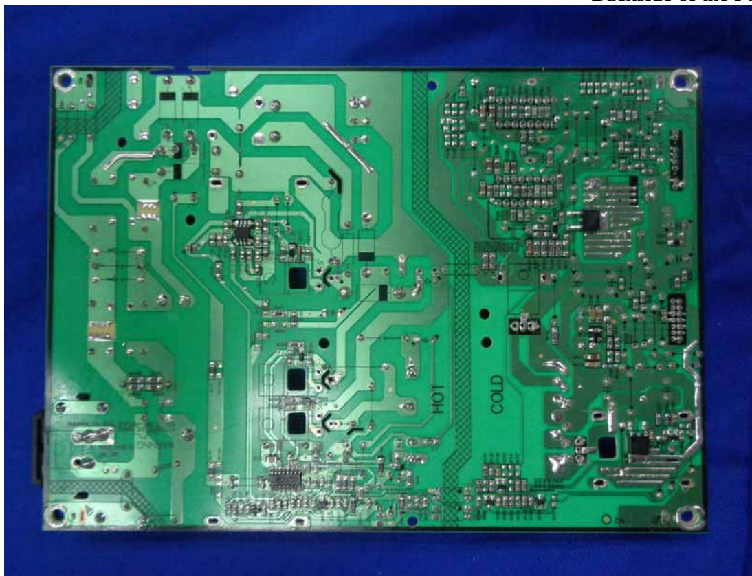
Figure 14 Backside of the Power Board
