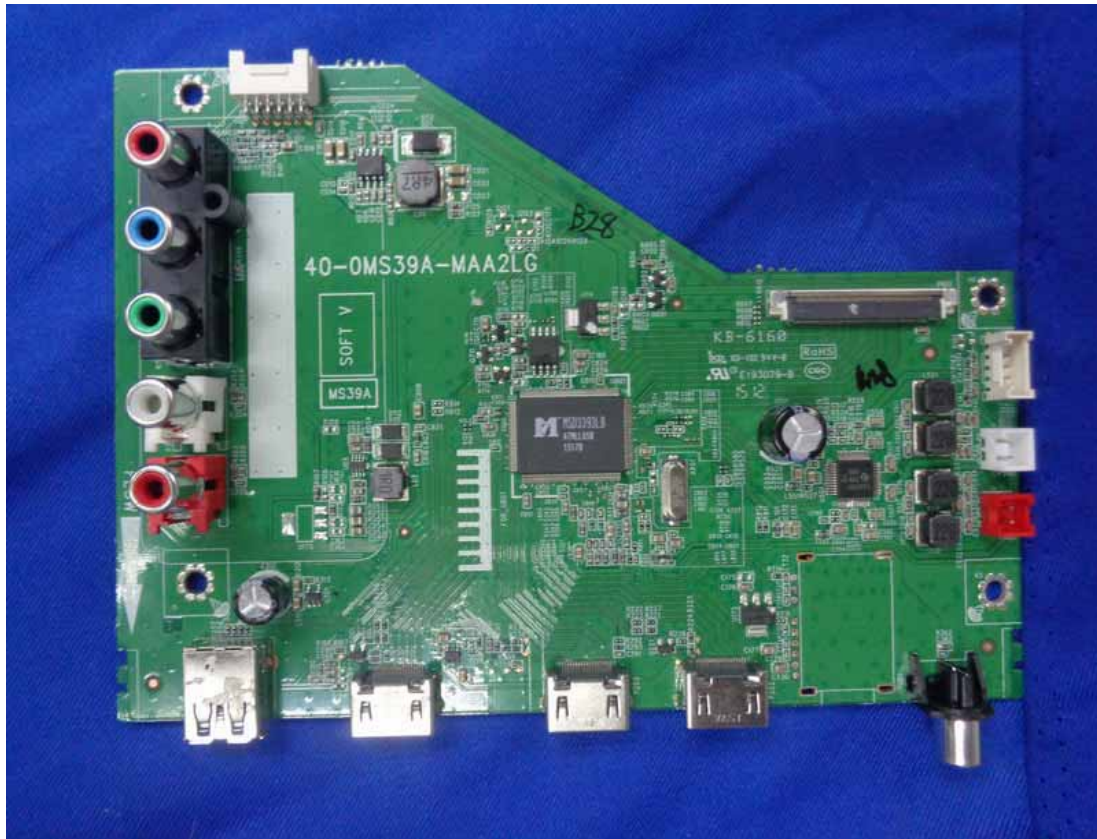
Figure 9 Frontside of the Main Board
