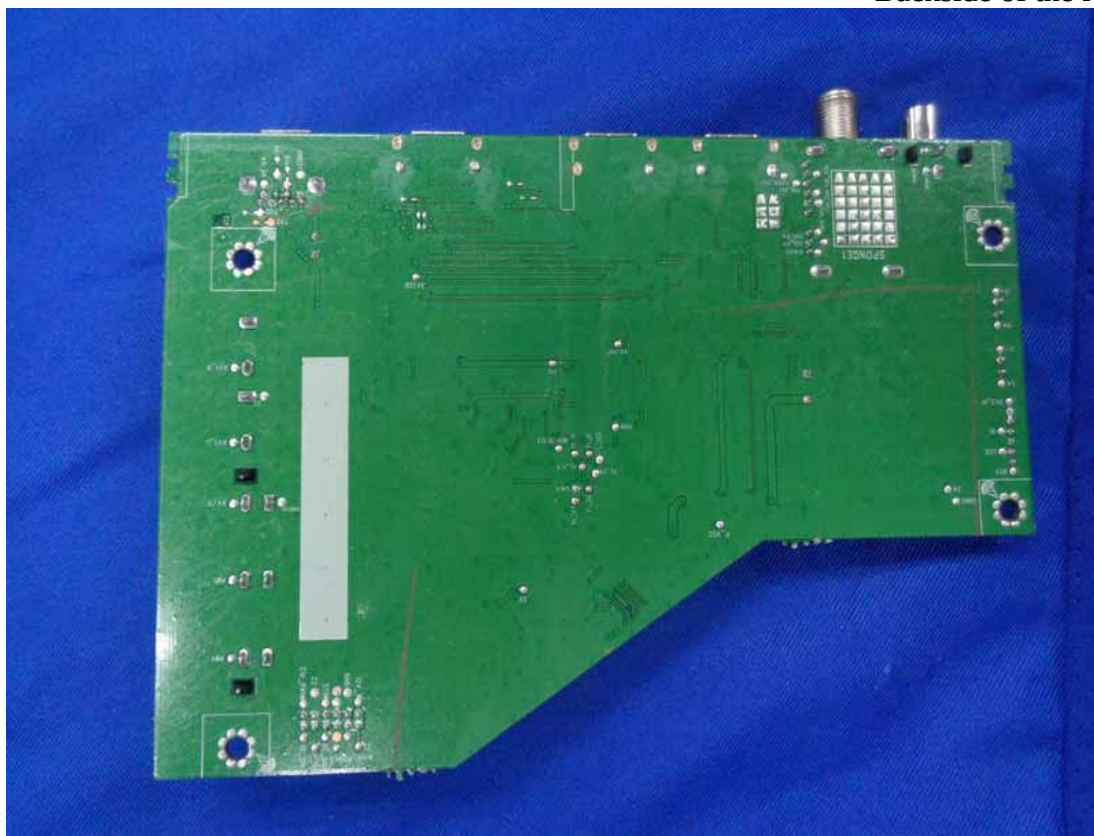
Figure 8 Backside of the Main Board
