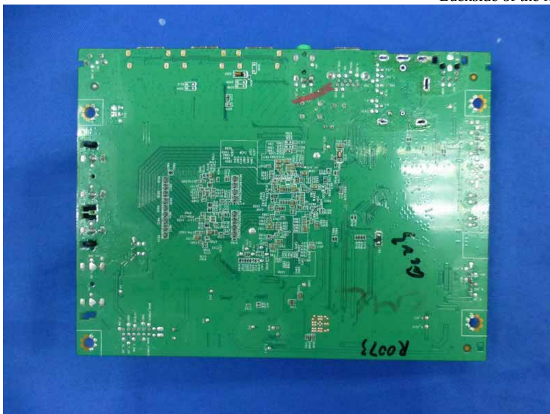
Figure 15 Backside of the Main Board
