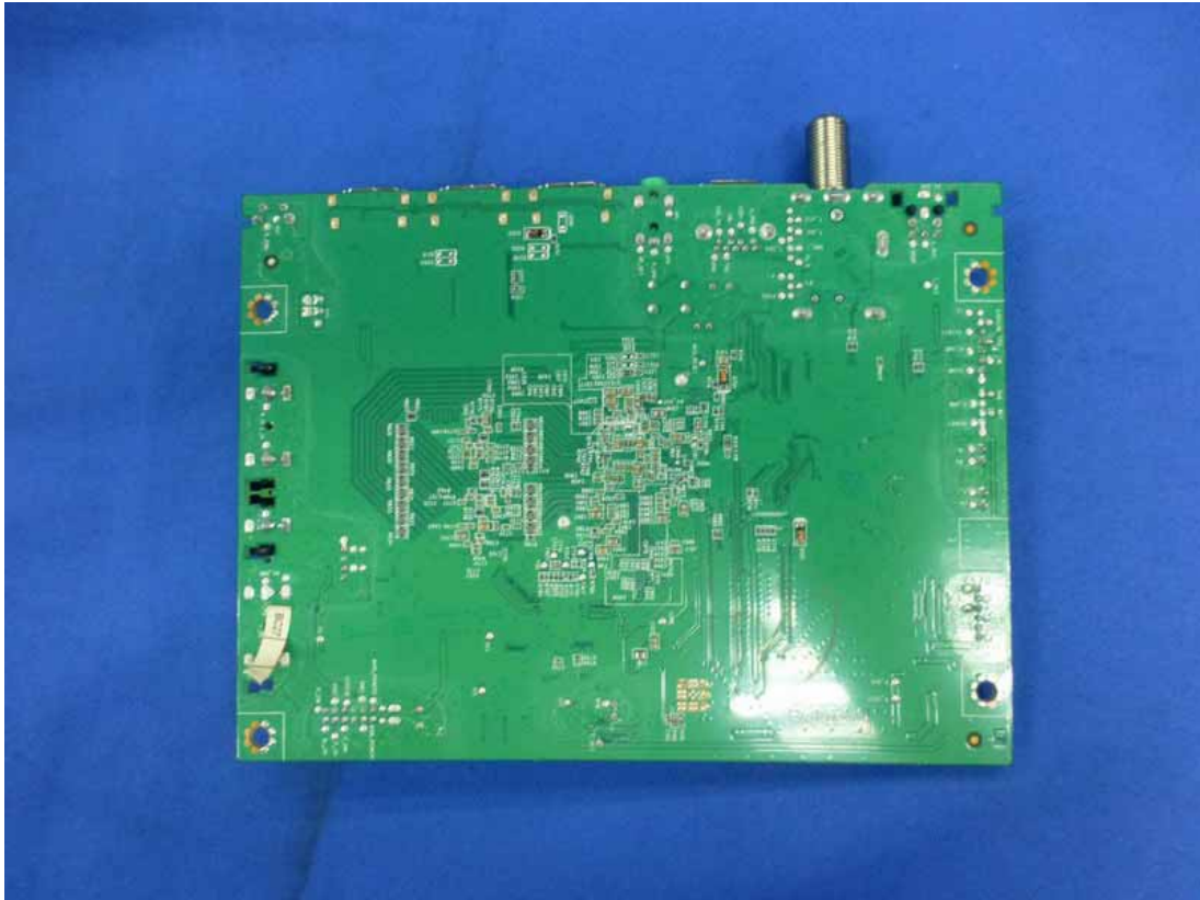
Figure 17 Backside of the Main Board
