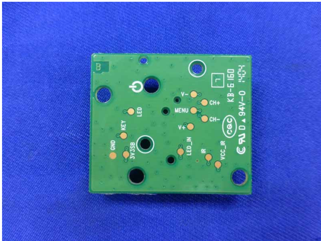
Figure 31 Backside of the PCB Board
