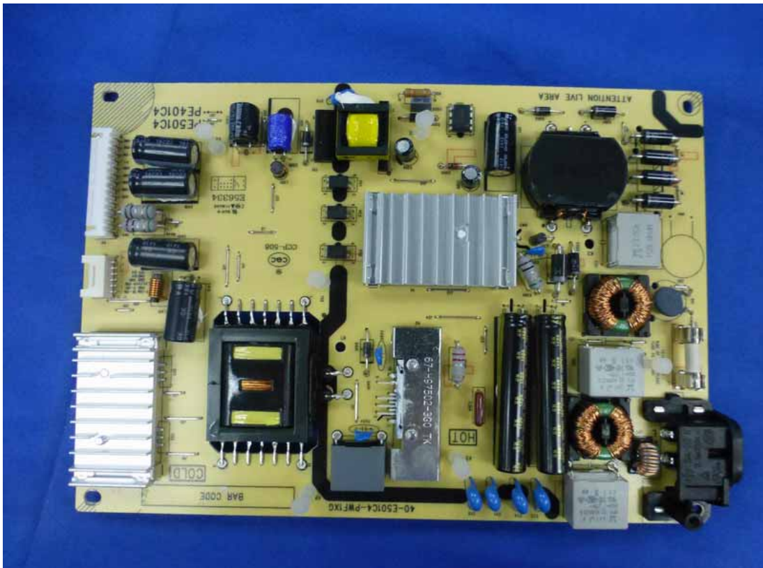
Figure 18 Frontside of the Power Board
