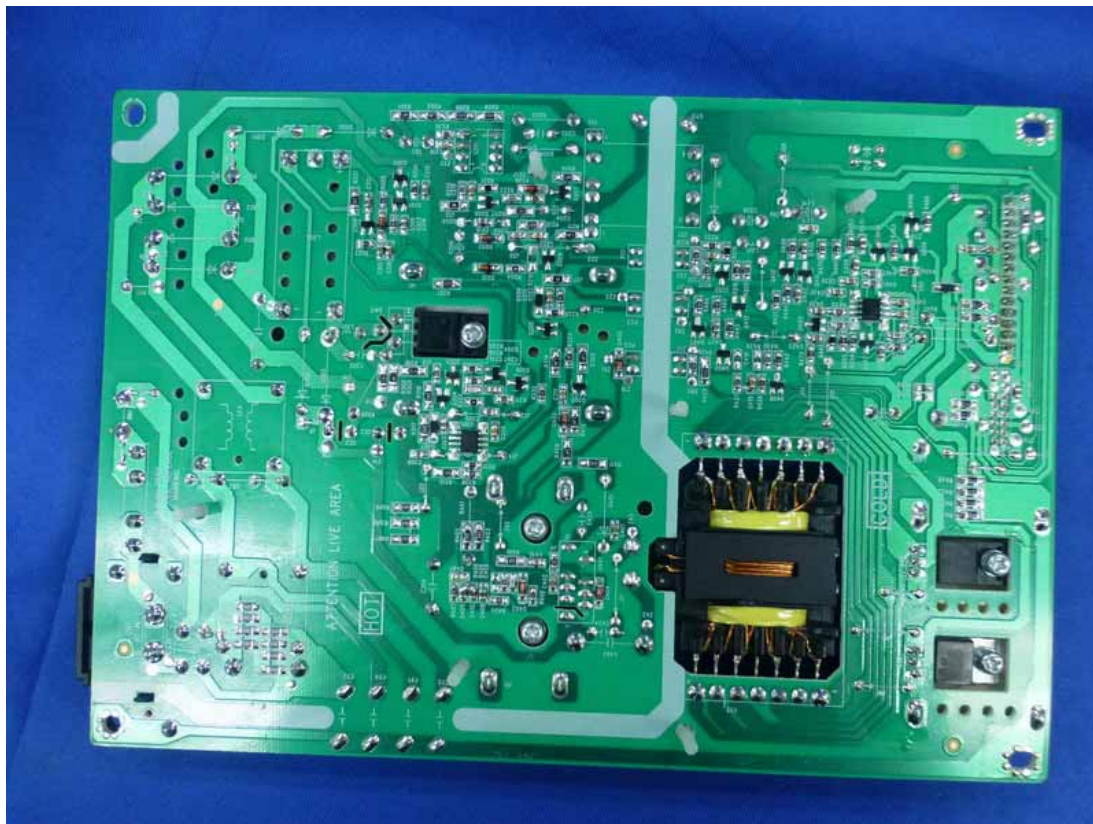
Figure 19 Backside of the Power Board
