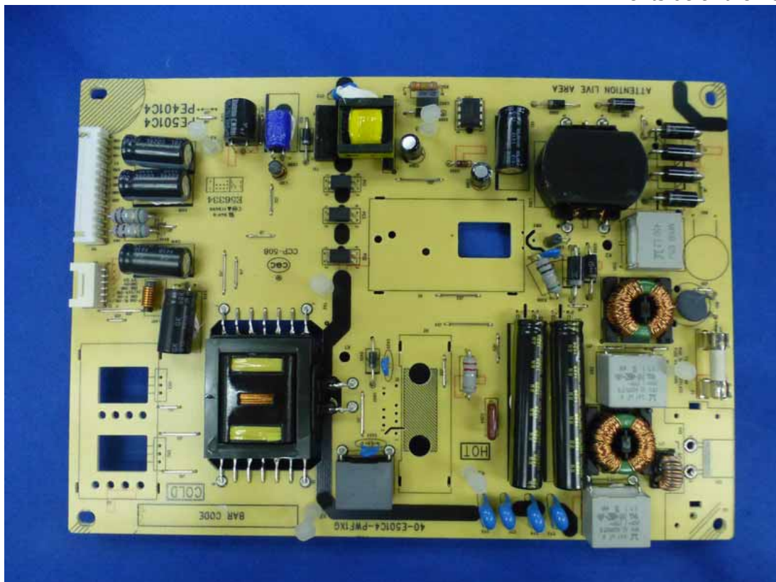
Figure 20 Frontside of the Power Board
