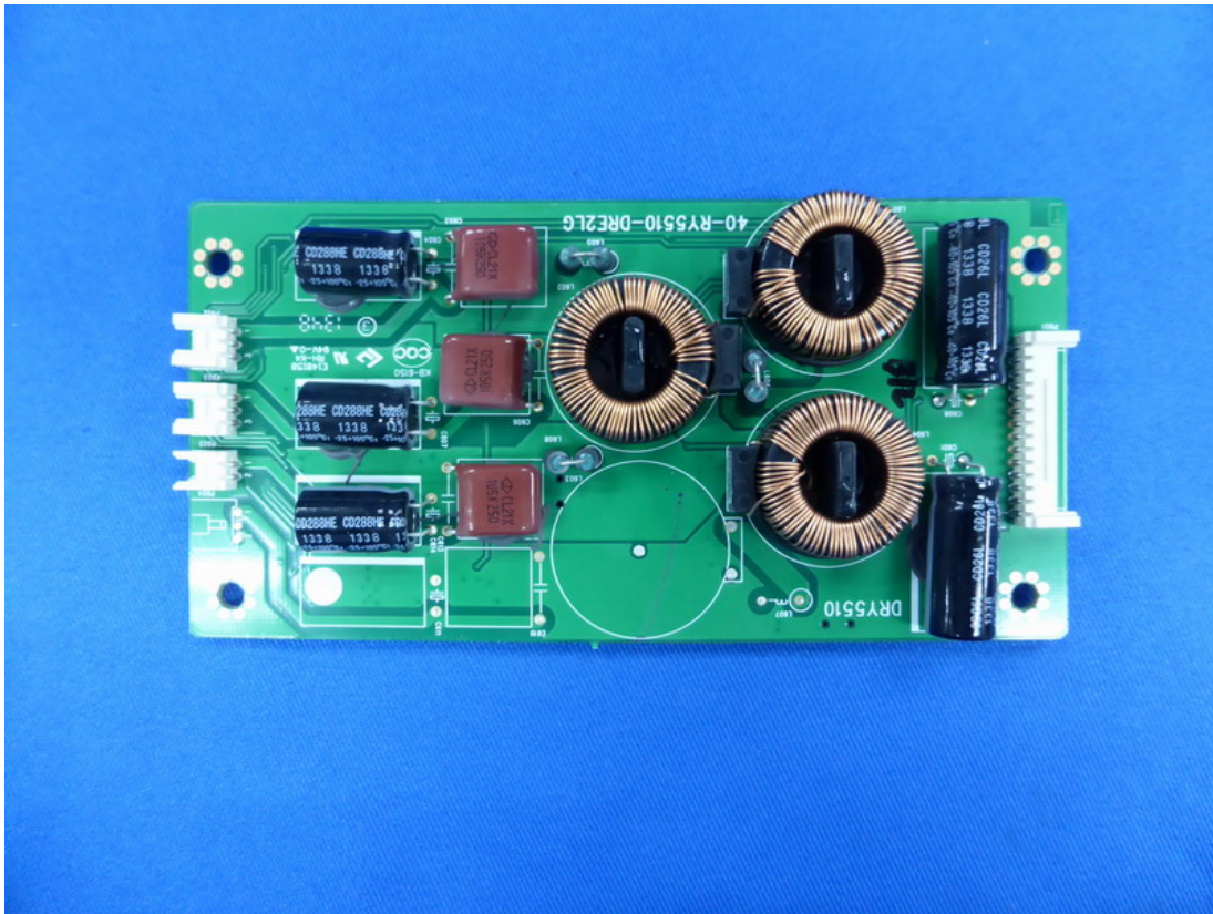
Figure 23 Frontside of the PCB Board
