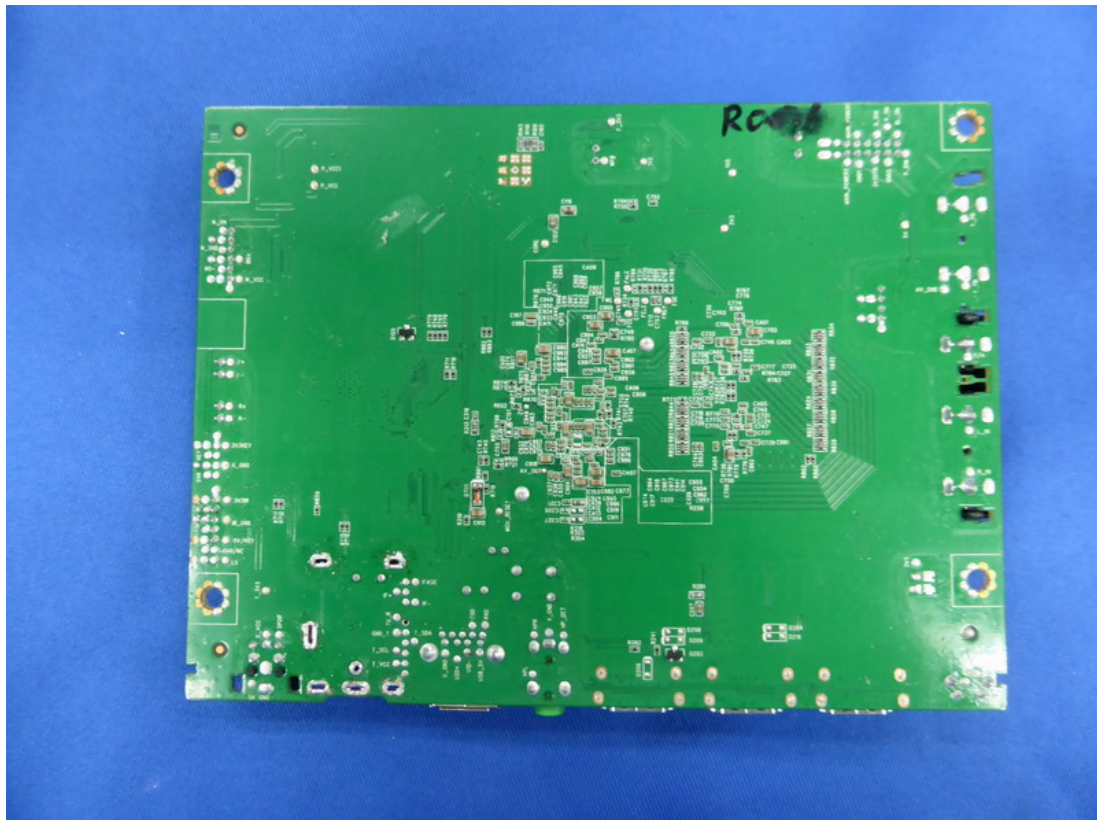
Figure 18 Backside of the Main Board
