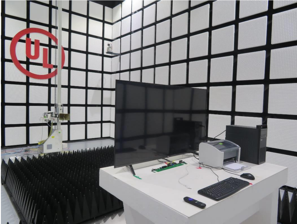
Radiated Disturbance above 1GHz – front view
