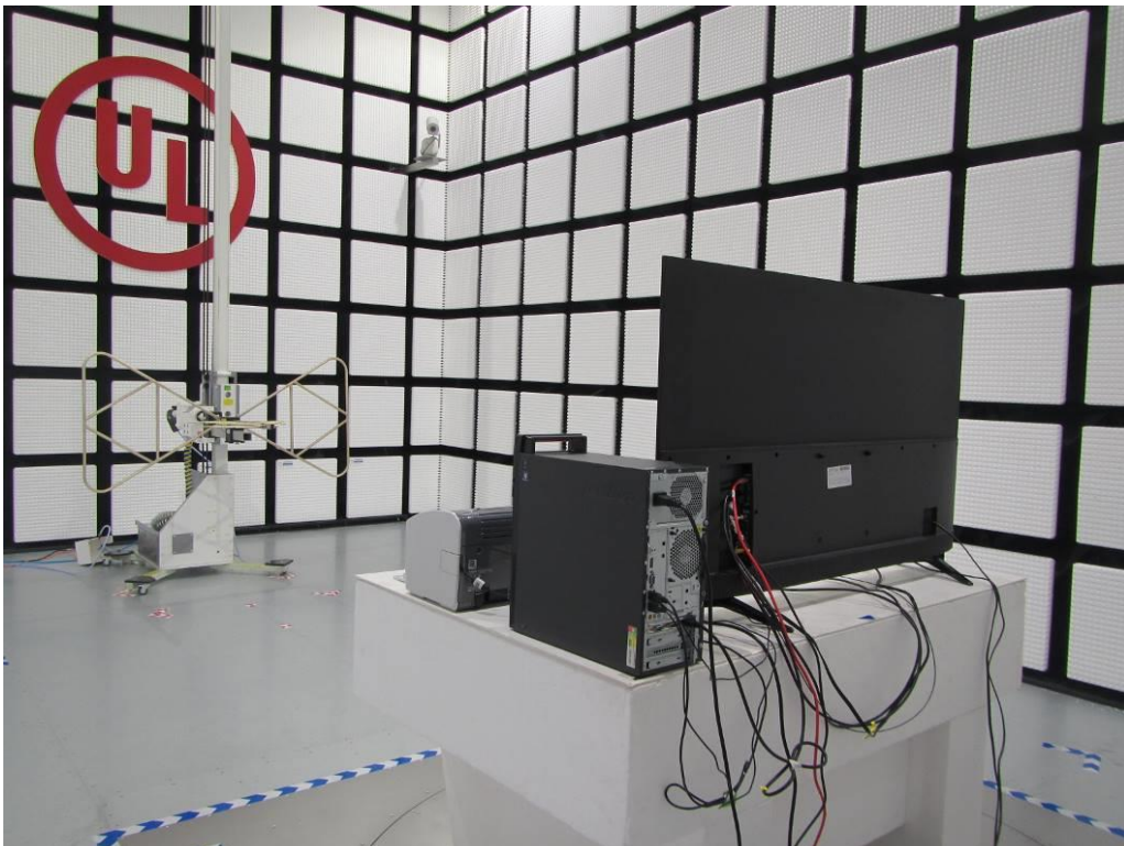
Radiated Disturbance below 1GHz – rear view
