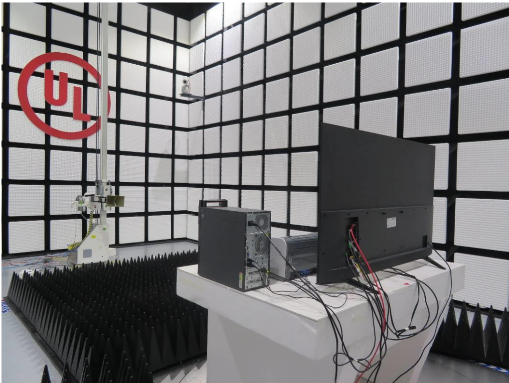
Radiated Disturbance above 1GHz – rear view
