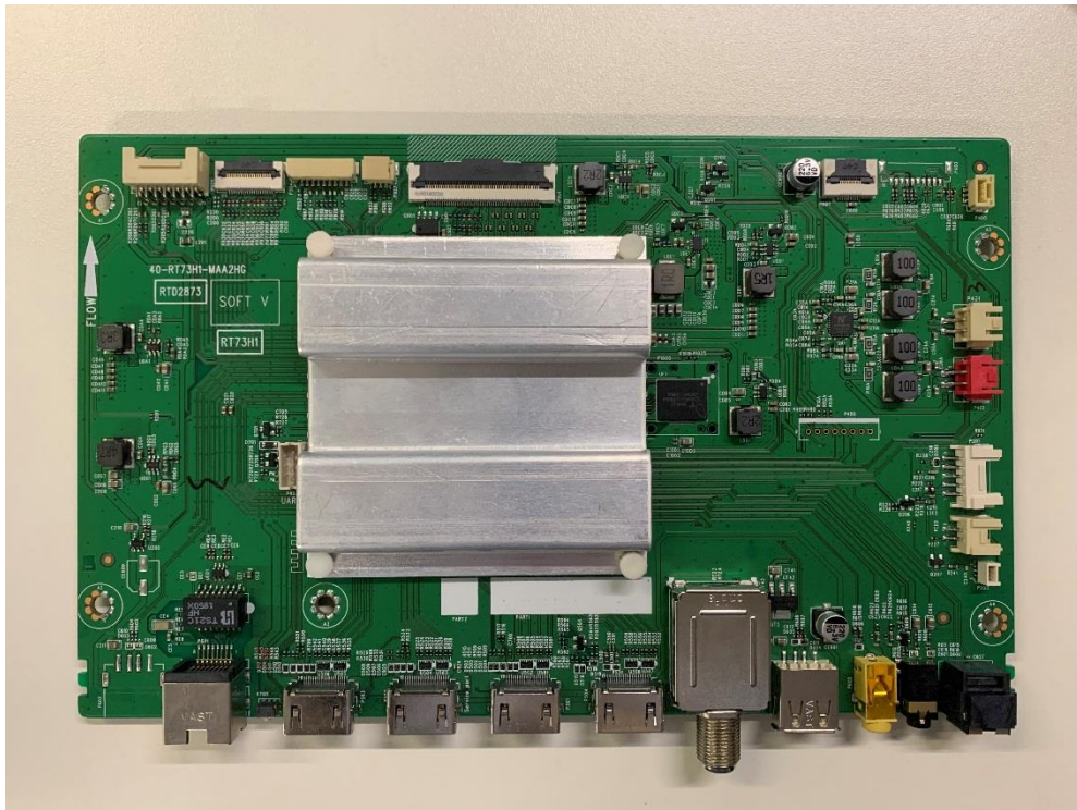
Mainboard with another heat sink
