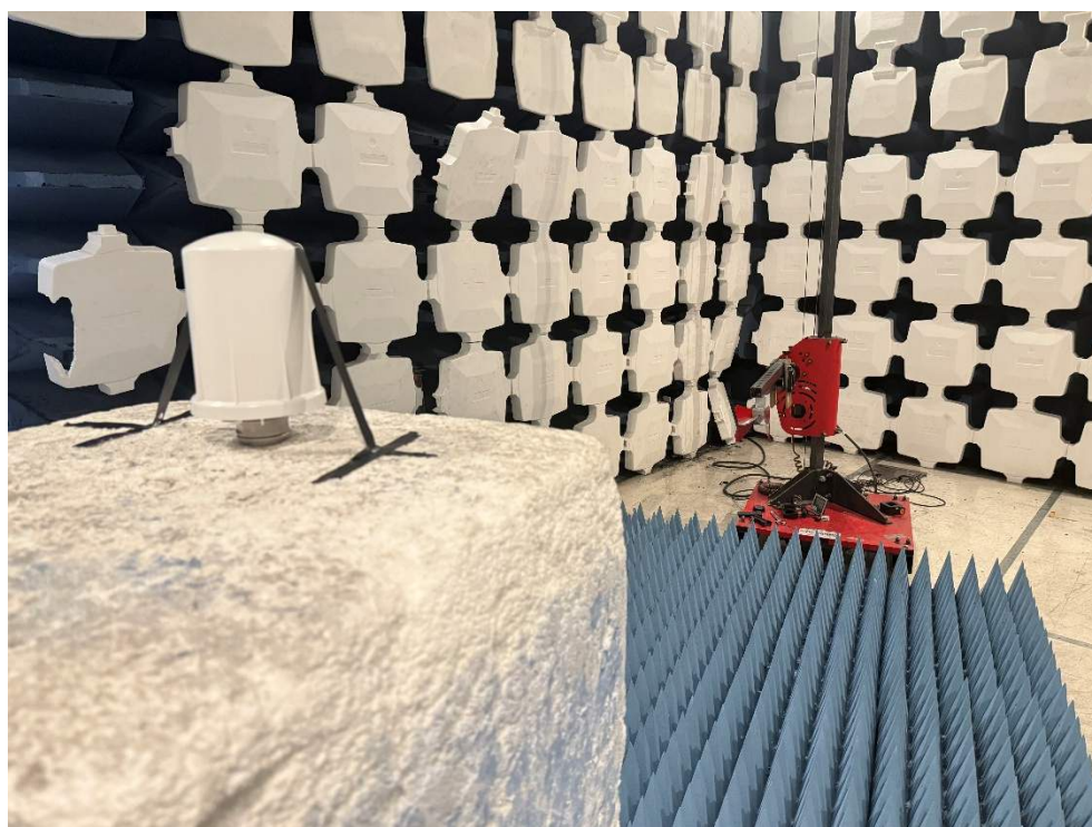
1-10GHz Rear
