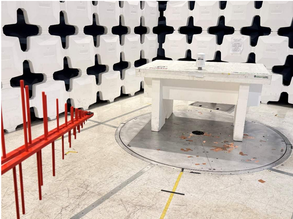
30MHz-1GHz Front
