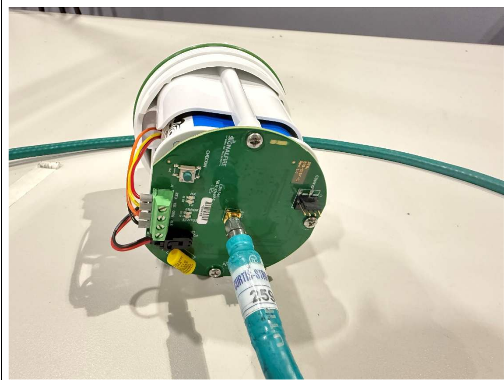
EUT Close-up
