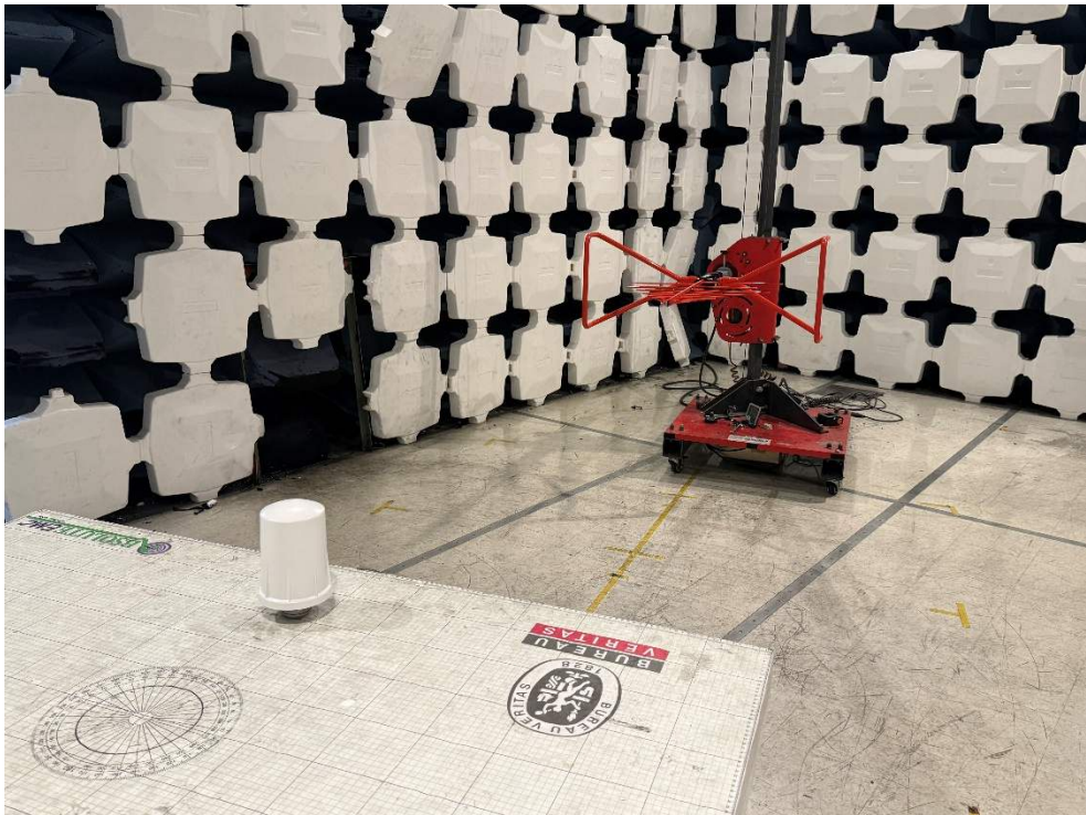
30MHz-1GHz Rear
