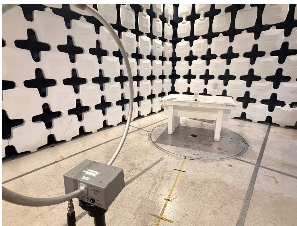
9kHz-30MHz Front
