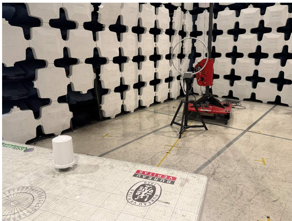
9kHz-30MHz Rear
