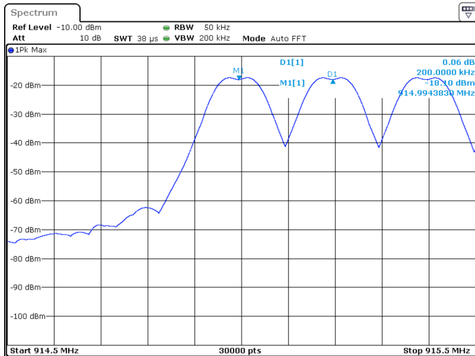
Channel Spacing - High Band - Low Edge
