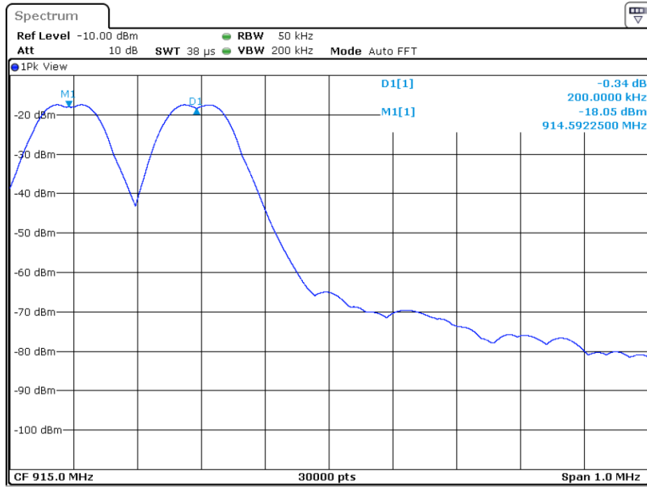
Channel Spacing - Low Band - High Edge
