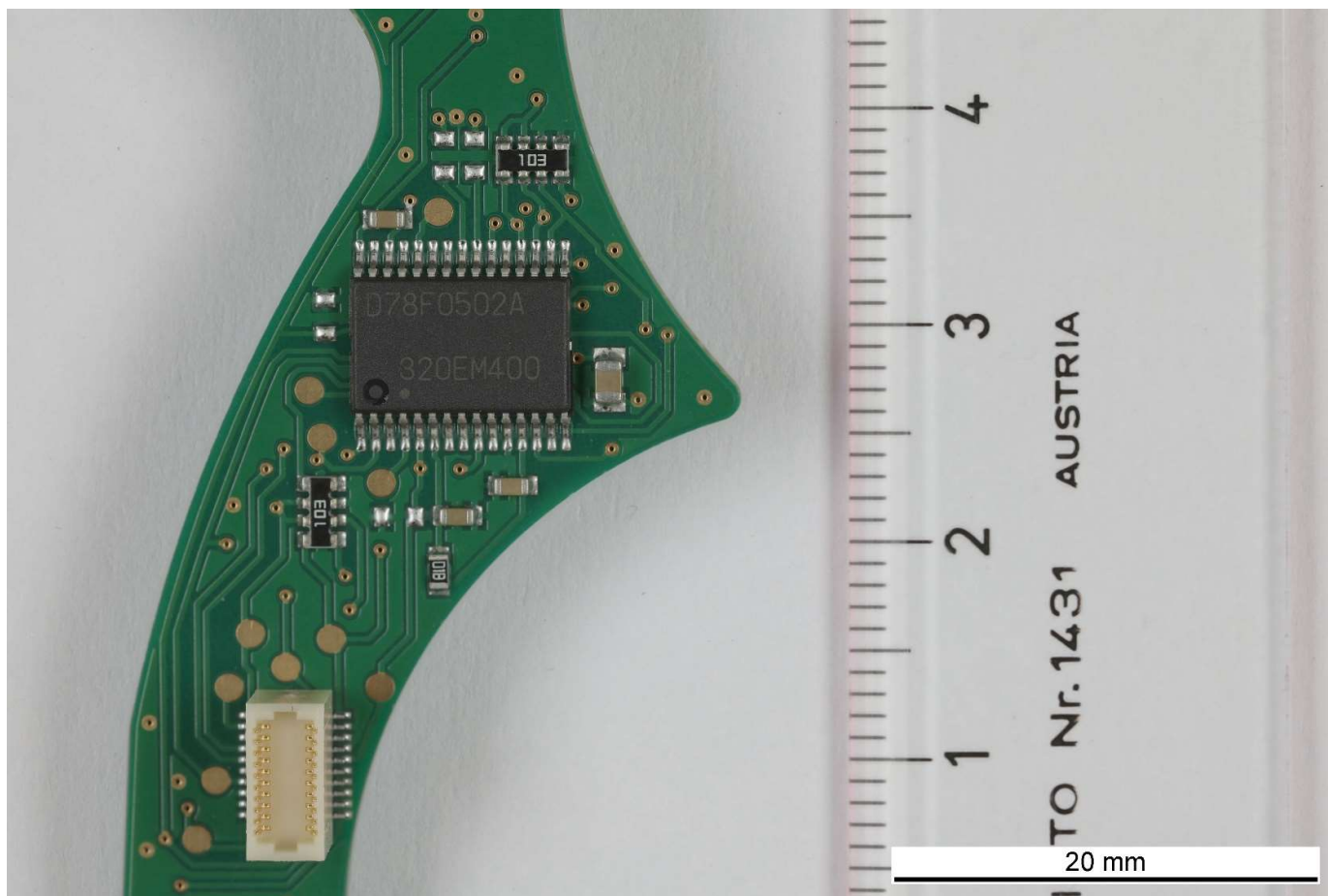
21.A00L31.02 Print: Front side detail view
