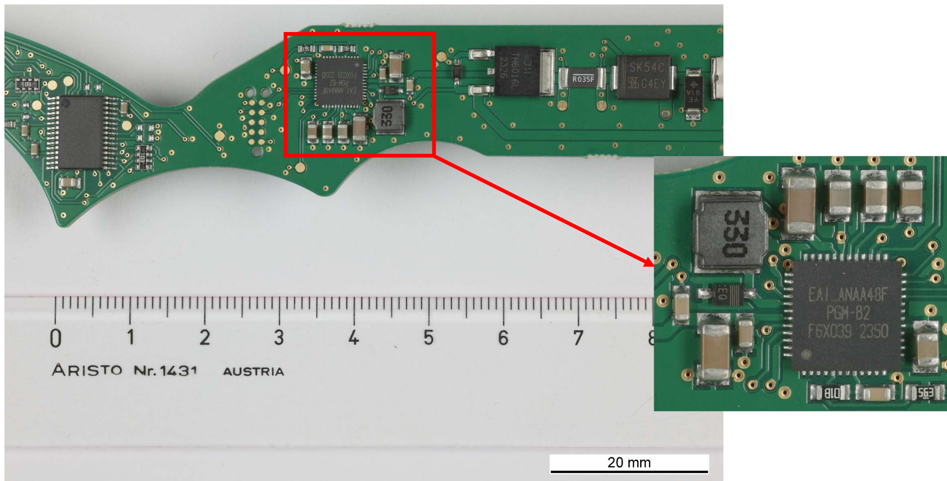
21.A00L31.02 Print: Front side detail view
