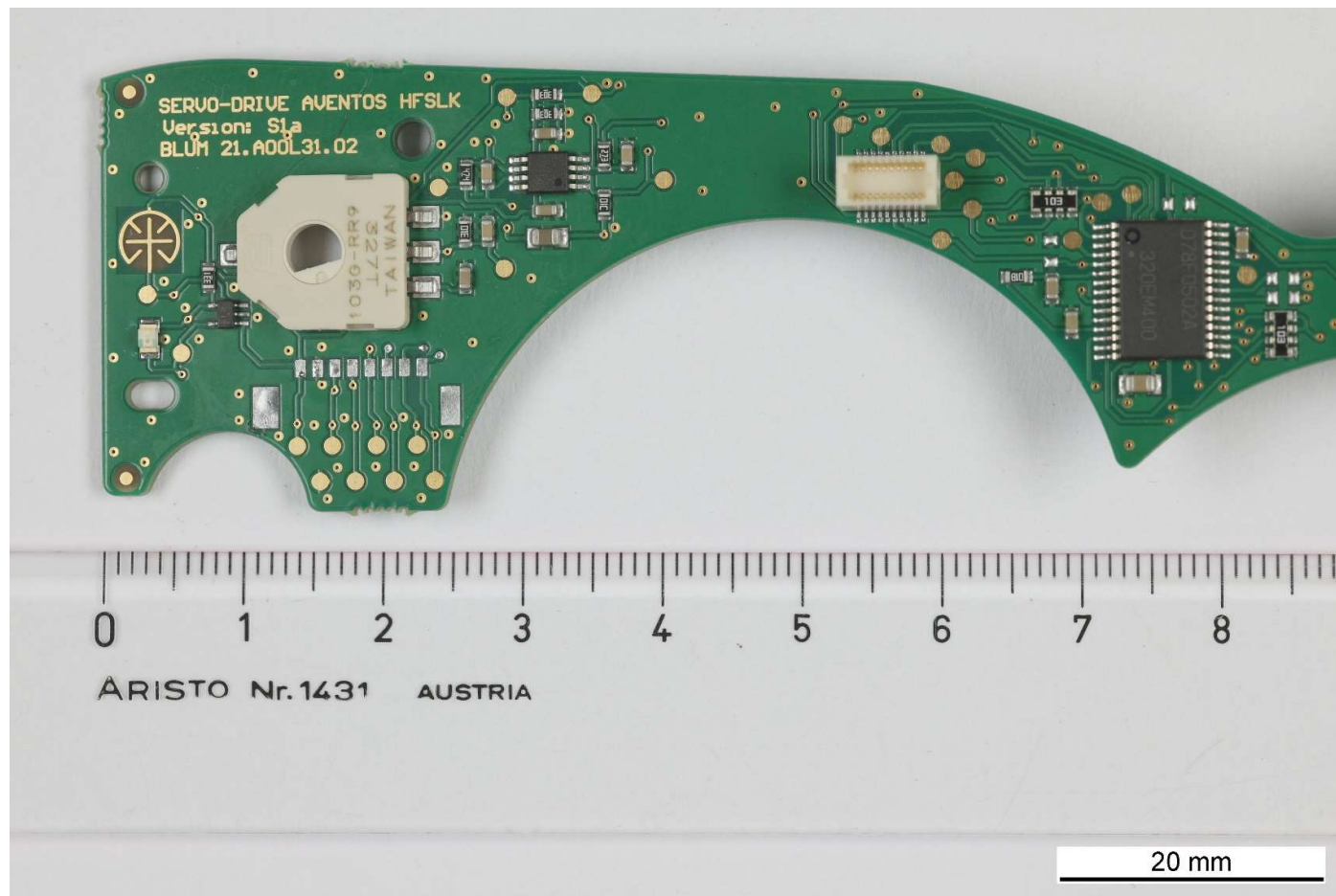
21.A00L31.02 Print: Front side detail view
