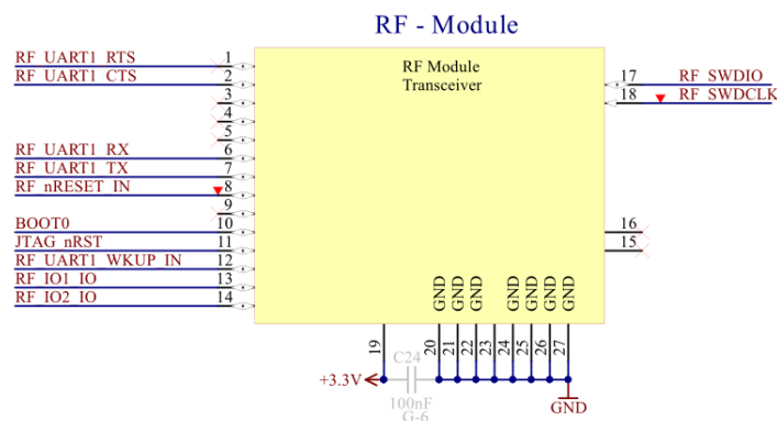
Image 2 Schematic
