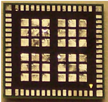
Back side of RF Transceiver
