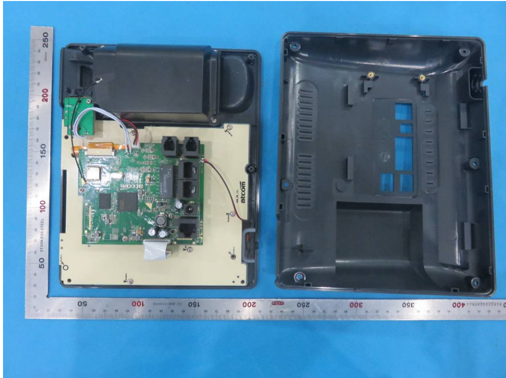
Model:A48W OPEN VIEW OF EUT
