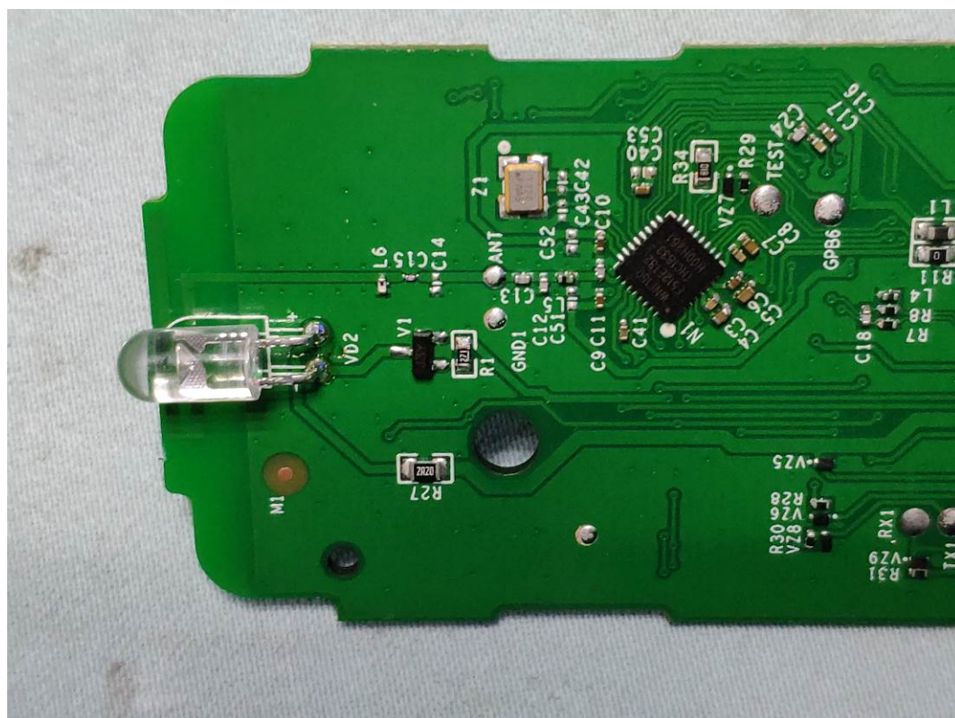
FIGURE 6 REMOTE CONTROL (M/N: ERF2A60) CHIP & CRYSTAL ON MAIN BOARD
