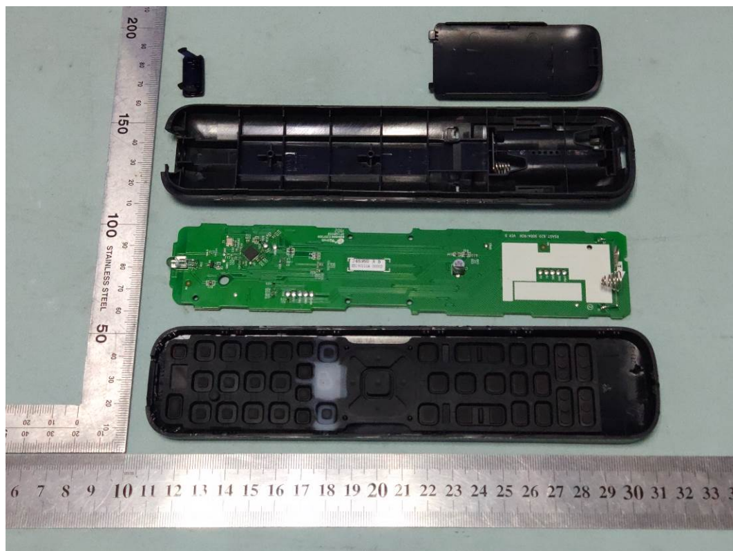
FIGURE 3 REMOTE CONTROL (M/N: ERF2A60) COVER REMOVED
