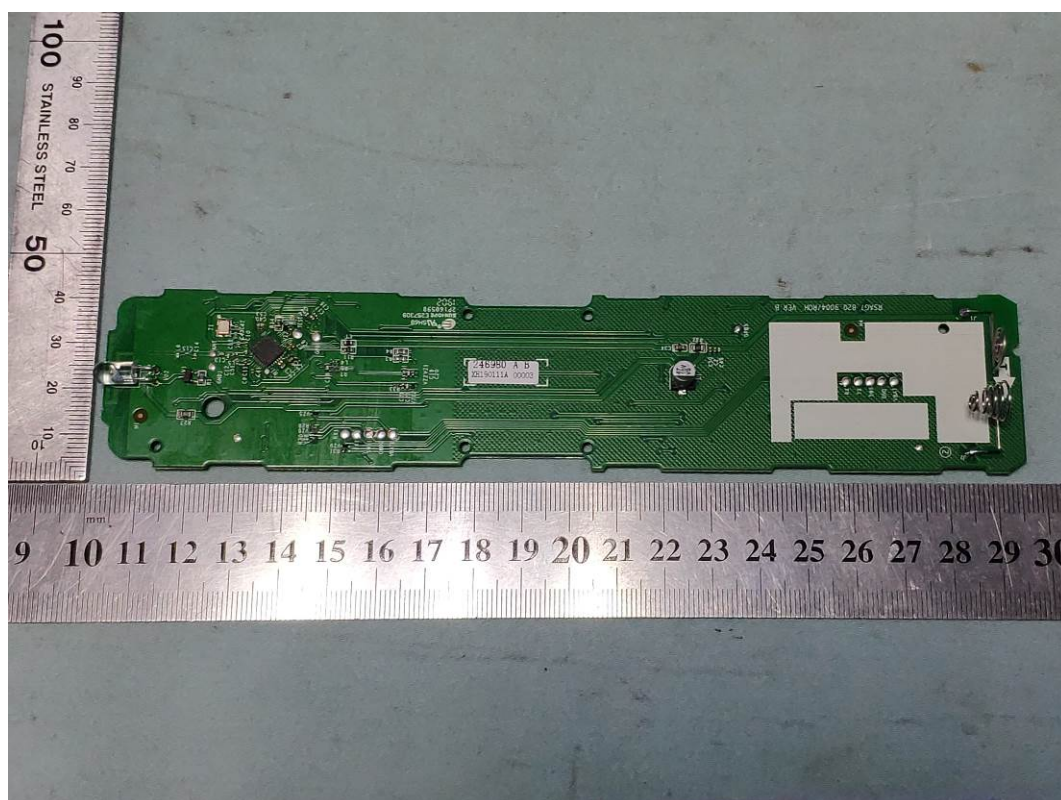
FIGURE 4 REMOTE CONTROL (M/N: ERF2A60) MAIN BOARD (COMPONENT SIDE)
