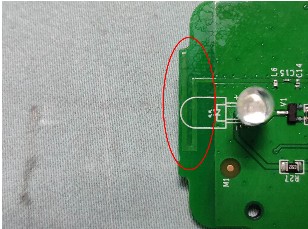
FIGURE 7 REMOTE CONTROL (M/N: ERF2A60) ANTENNA
