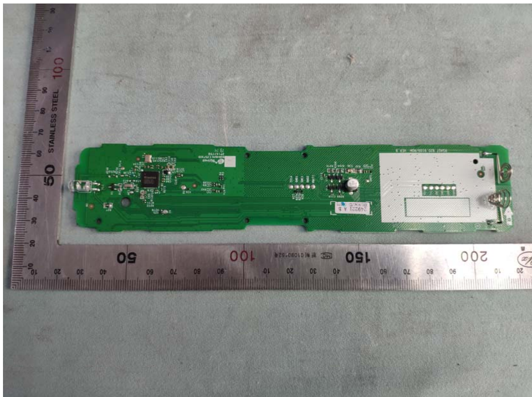
FIGURE 4 REMOTE CONTROL (M/N: ERF2A60(1001)) MAIN BOARD (COMPONENT SIDE)
