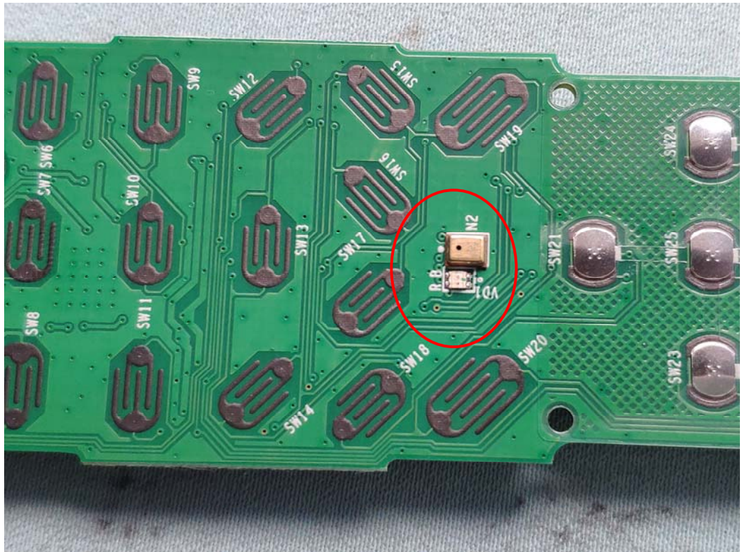
FIGURE 7 REMOTE CONTROL (M/N: ERF2A60(1001)) MICROPHONE
