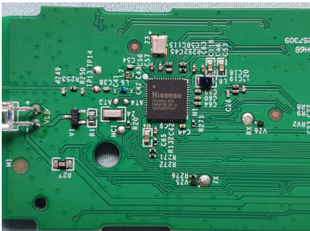
FIGURE 6 REMOTE CONTROL (M/N: ERF2A60(1001)) CHIP & CRYSTAL ON MAIN BOARD
