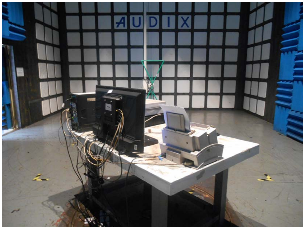
SETUP WITH MAXIMUM DETECTED EMISSION AT VERTICAL POLARIZATION (TEST MODE: HDMI 1280*1024@60Hz & 1kHz PLAYING)
