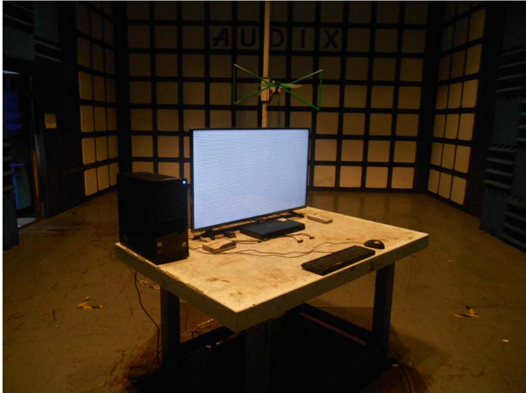
SETUP WITH MAXIMUM DETECTED EMISSION AT HORIZONTAL POLARIZATION (TEST MODE HDMI1 1280*1024@60Hz & 1kHz PLAYING)
