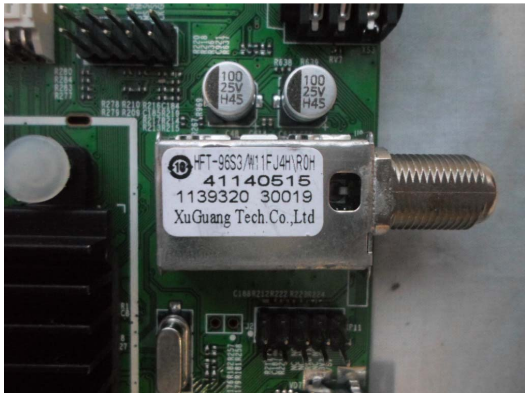
FIGURE 9 LED LCD TV (M/N: 50H4) TUNER ON MAIN BOARD
