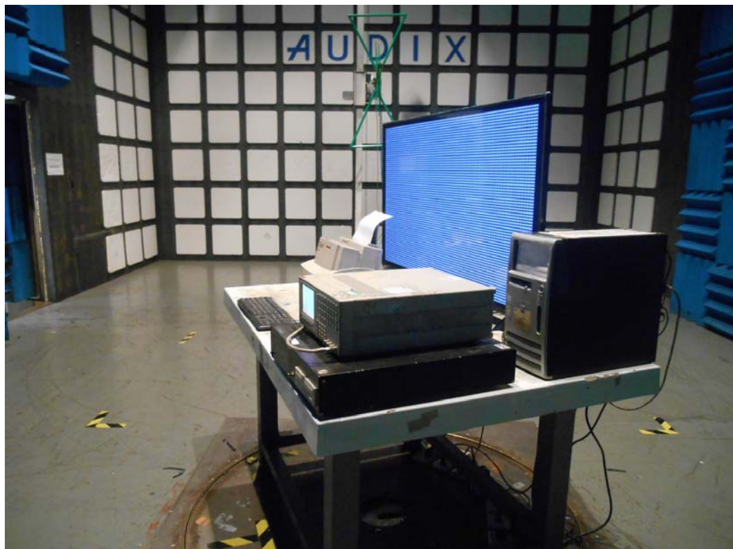
SETUP WITH MAXIMUM DETECTED EMISSION AT VERTICAL POLARIZATION (TEST MODE: HDMI 1280*1024@75Hz & 1kHz PLAYING)
