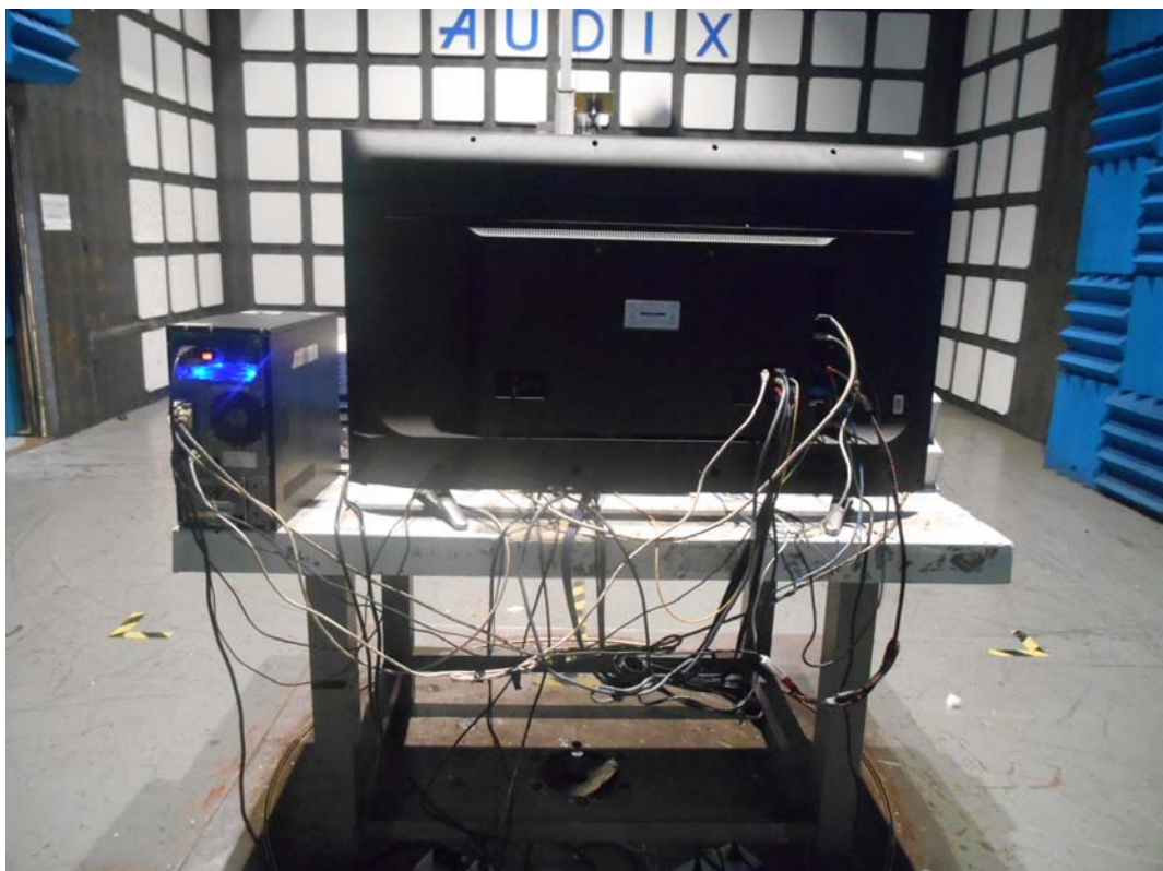
BACK VIEW OF RADIATED EMISSION TEST (HIGH 1GHz)
