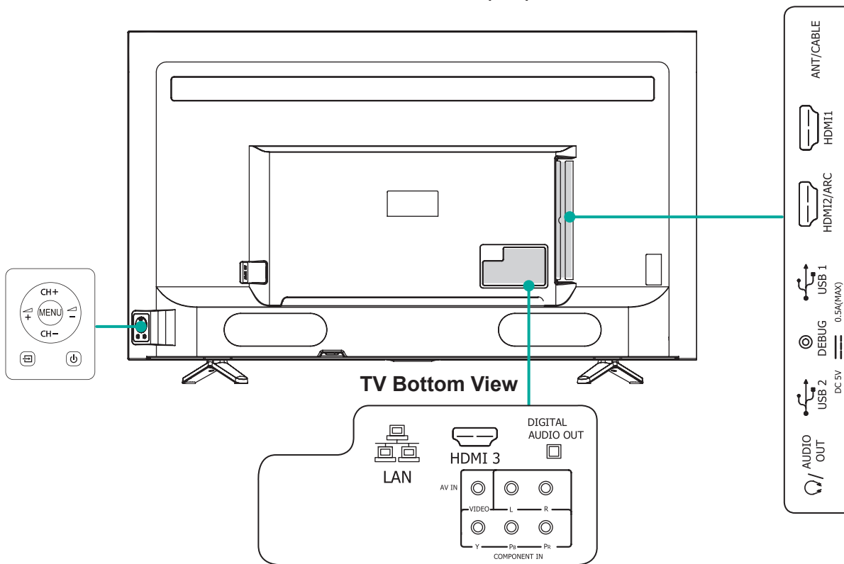
Back View of the TV (50")
