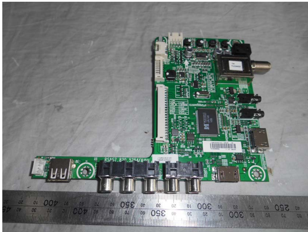
FIGURE 5 LED LCD TV (M/N: LC-50N3100U) MAIN BOARD (COMPONENT SIDE)
