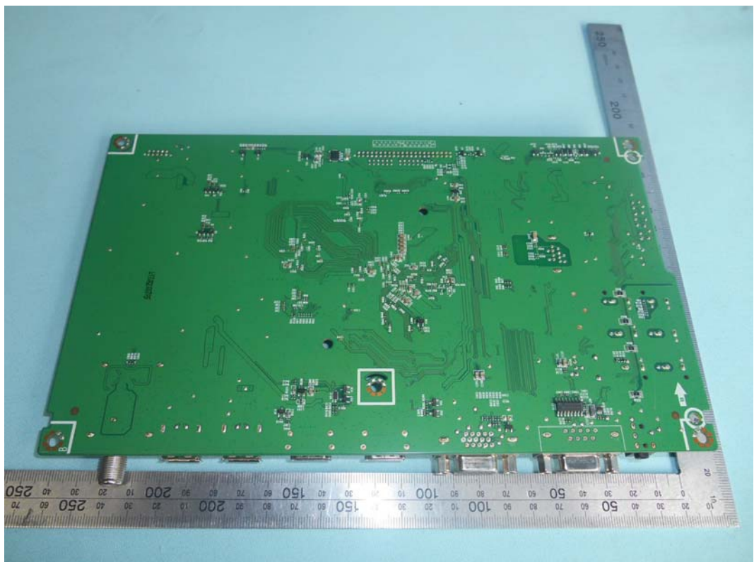
FIGURE 6 LED LCD TV (M/N: LC-55F) MAIN BOARD (SOLDERED SIDE)
