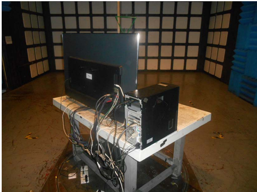
SETUP WITH MAXIMUM DETECTED EMISSION AT VERTICAL POLARIZATION (TEST MODE: HDMI4 3840*2160@60Hz & 1kHz PLAYING)
